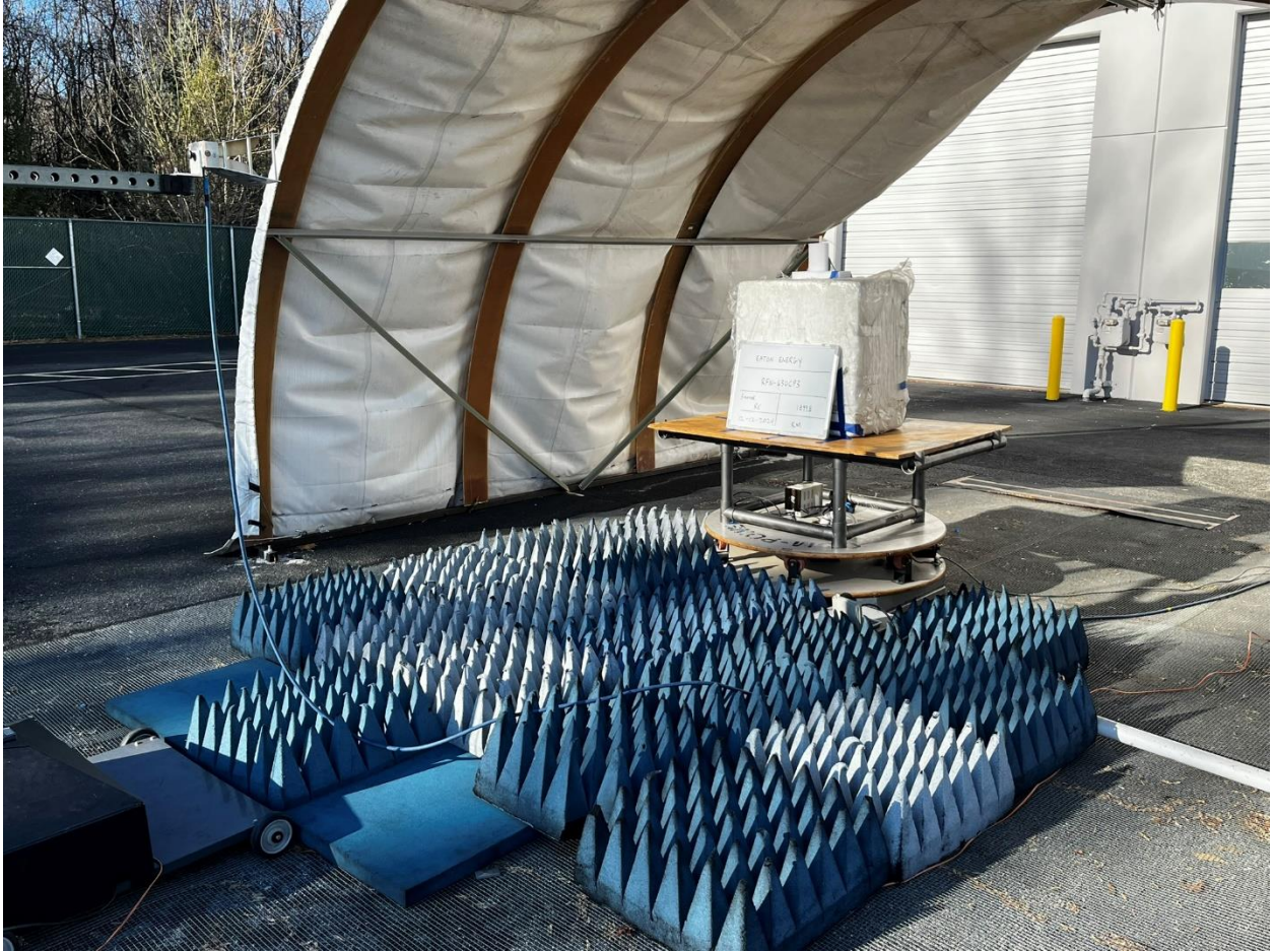
RE > 1GHz Front 1
