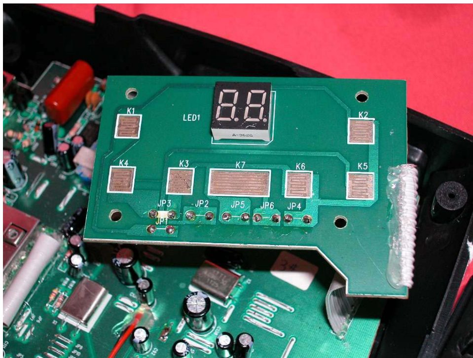
Base DAM PCB comp side
