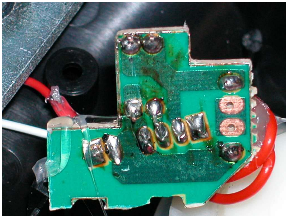
Corded Handset receiver volume PCB solder side
