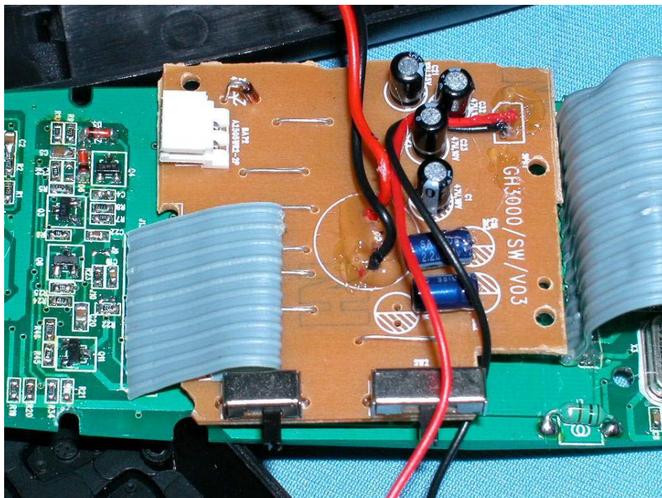
Handset another PCB comp side
