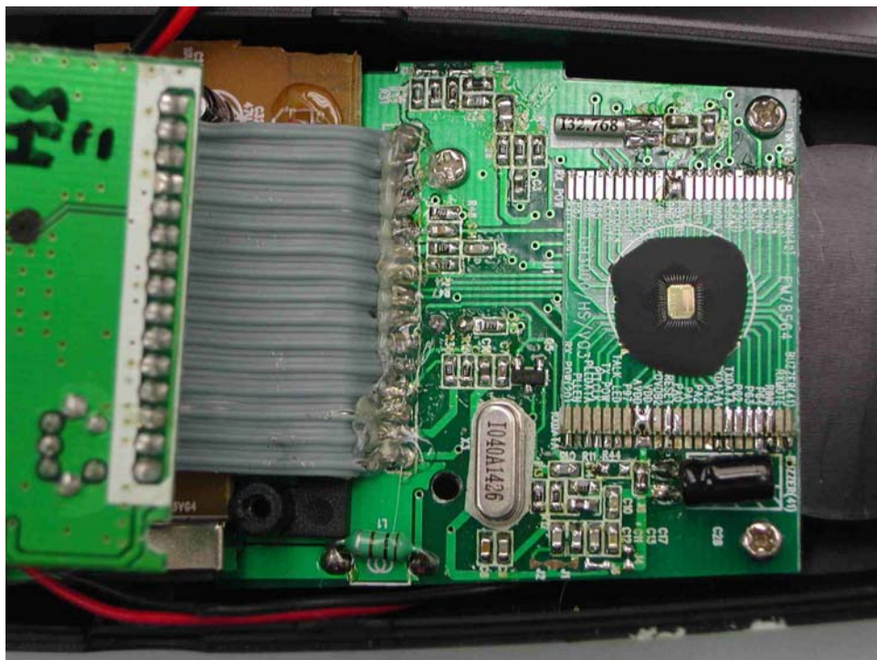
Handset Main PCB comp side (View 4)
