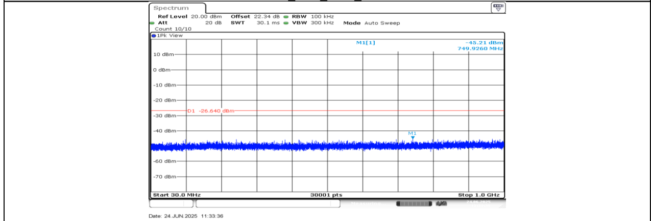
11N20SISO_Ant1_2462_30~1000
