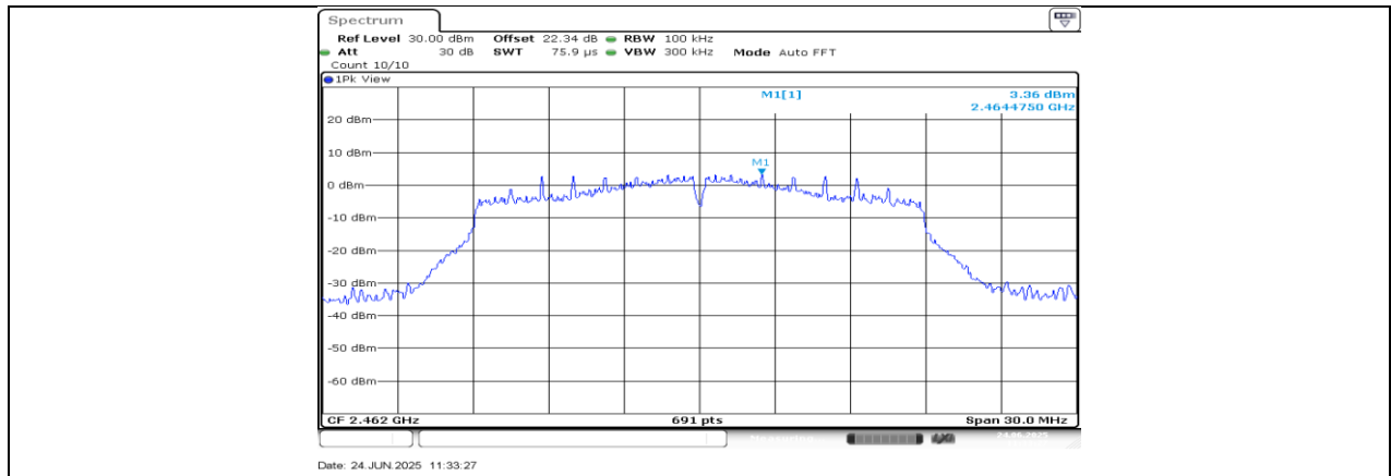
11N20SISO_Ant1_2462_0~Reference
