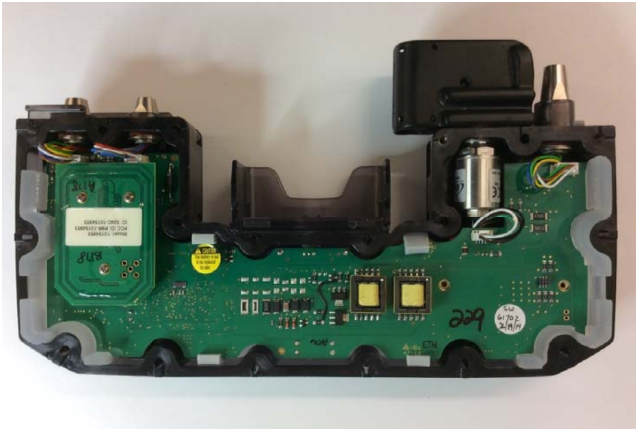
Figure 1 - RFID PCBA Placement on Power Module
