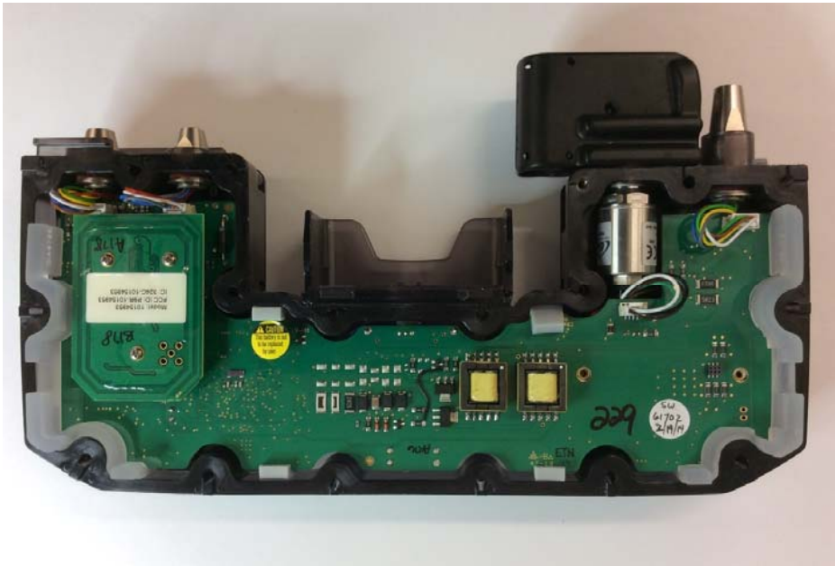
Figure 7 - RFID PCBA Placement on Power Module
