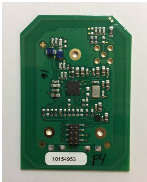
Figure 2 - RFID PCBA (Top)
