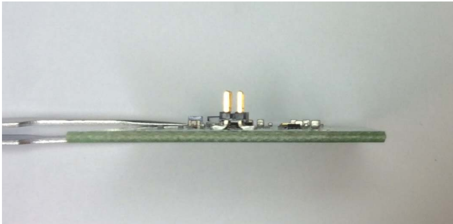
Figure 5 - RFID PCBA (Side #3)
