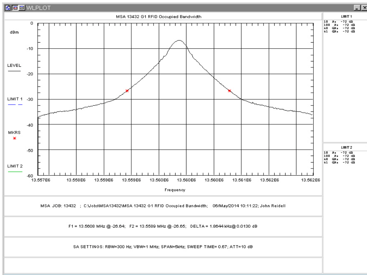
Figure 2: Occupied Bandwidth
