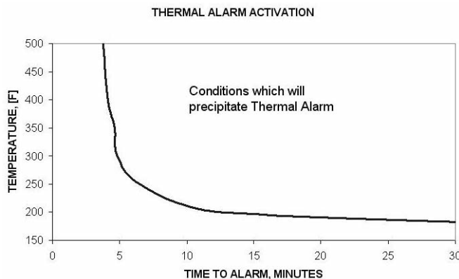
Chart 3: FireHawk M7 Control Module Thermal Alarm Activation Curve
