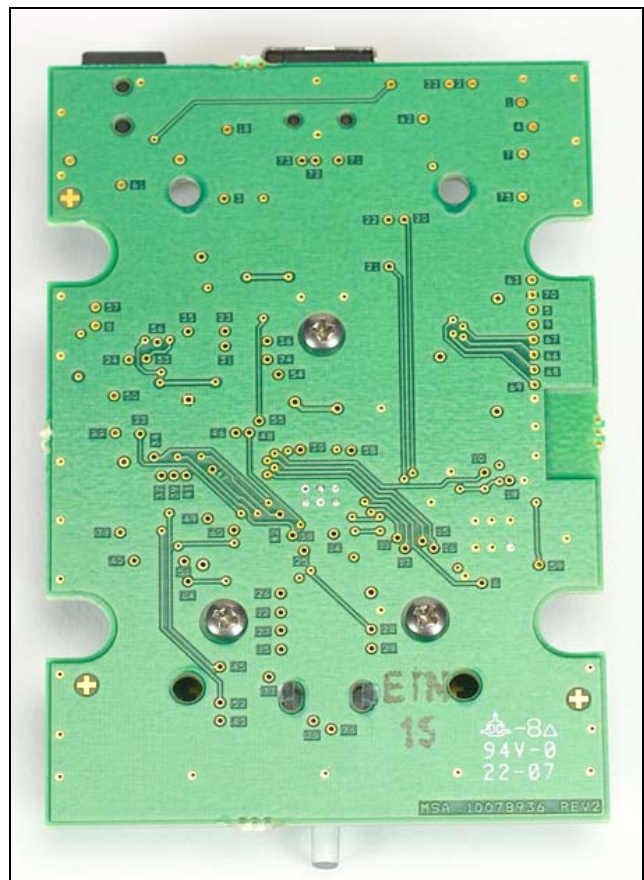
Board Bottom
