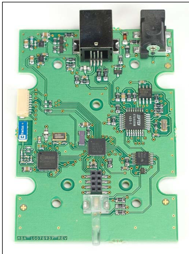
Reader / ID Tag writer – Board Top
