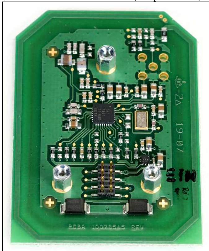
Front (component side)
