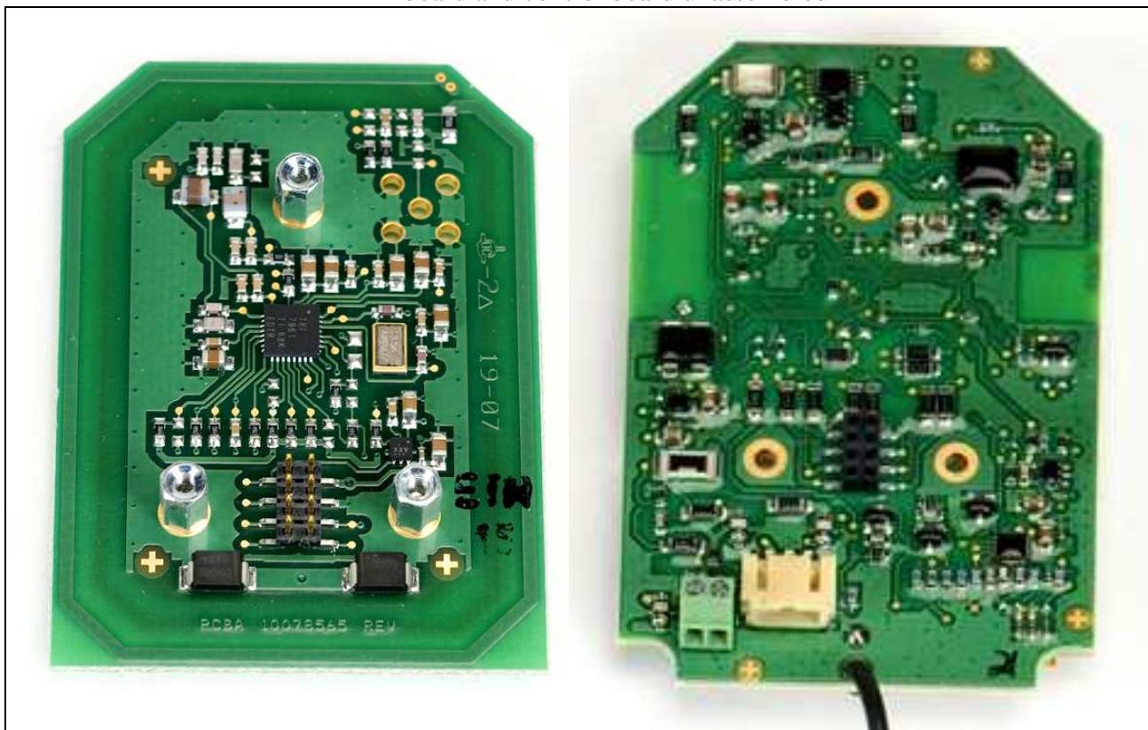
RFID board and control board unassembled
