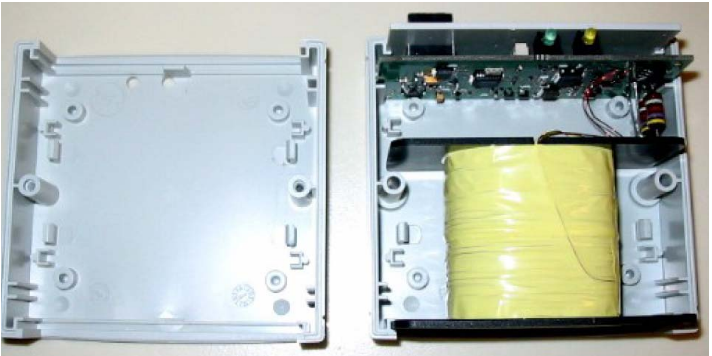
Tag Writer Internal Photos
