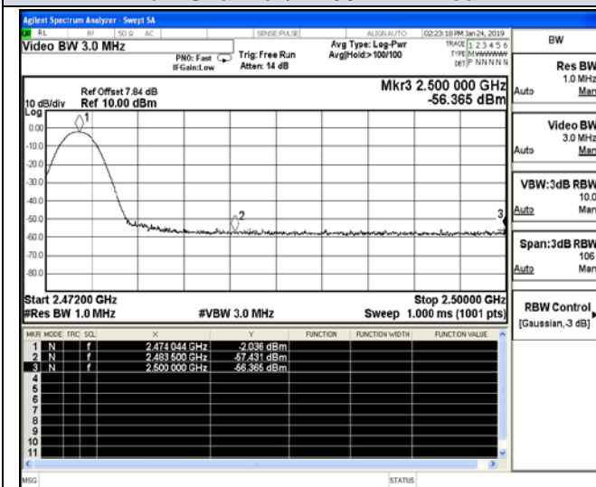
High Channel / 2474MHz - Peak
