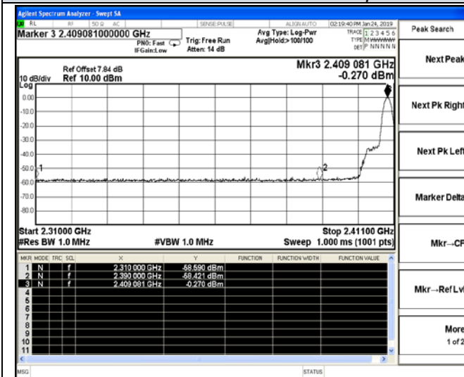
Low Channel / 2409MHz - Peak
