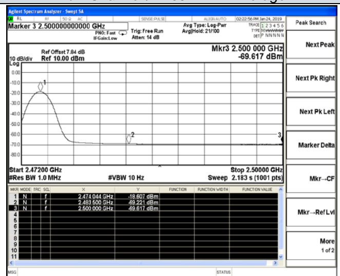
High Channel / 2474MHz - Average
