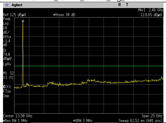
2437MHz_40MHz_n-mode_Peak_Ant B
