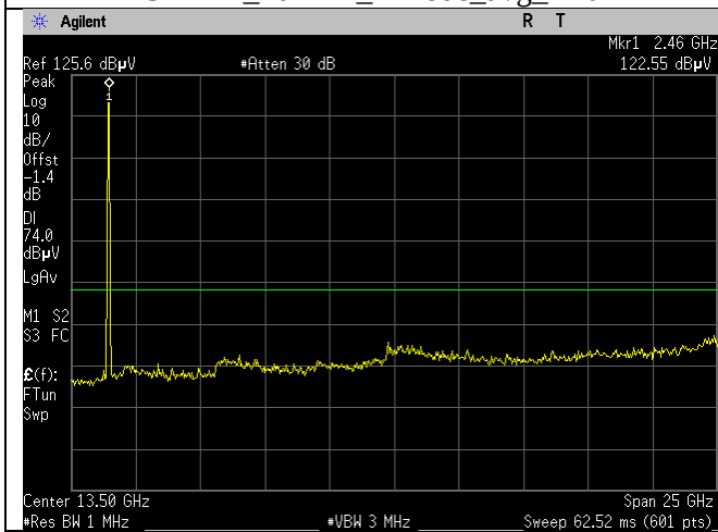
2437MHz_40MHz_n-mode_Peak_Ant A
