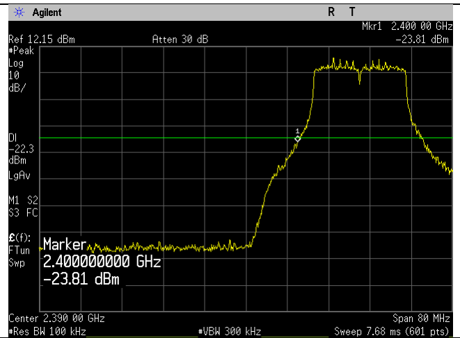
2412MHz_20MHz_n-mode_Lower Band Edge_Ant B
