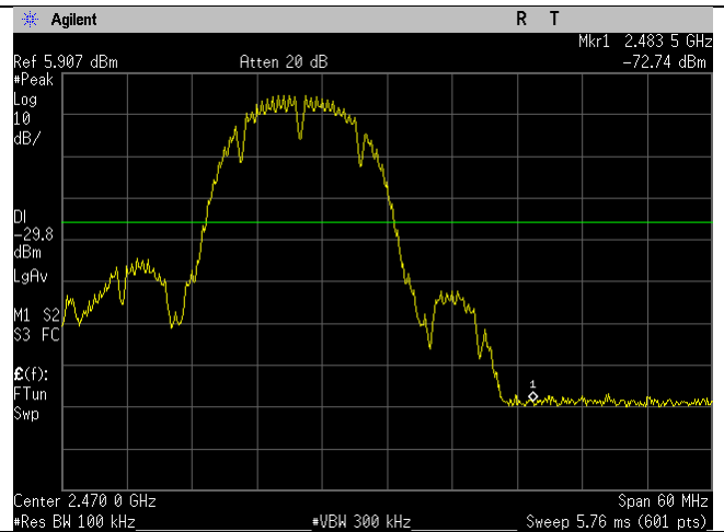
2462MHz_20MHz_b-mode_Upper Band Edge_Ant B
