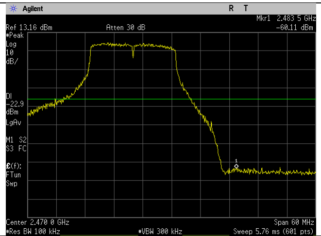
2462MHz_20MHz_n-mode_Upper Band Edge_Ant B
