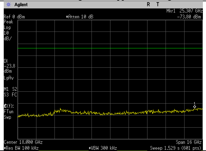
2462MHz_20MHz_n-mode_10-26GHz_Ant B
