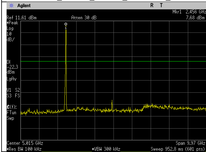
2462MHz_20MHz_n-mode_30MHz-10GHz_Ant A
