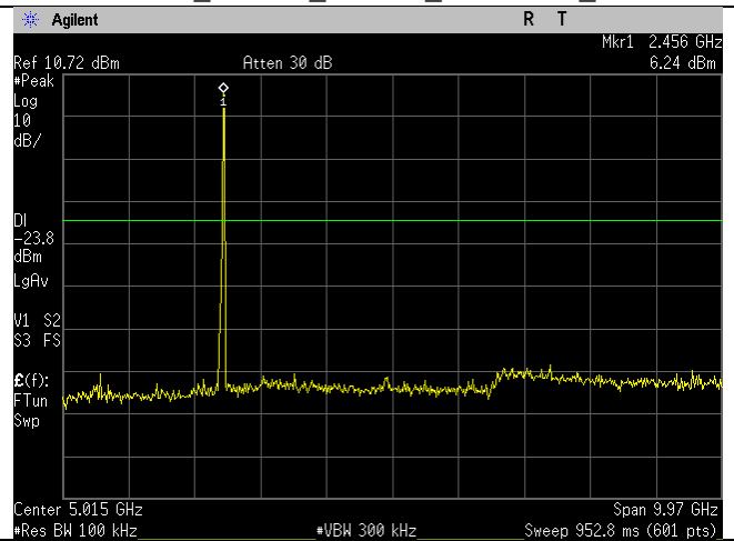
2462MHz_20MHz_n-mode_30MHz-10GHz_Ant B
