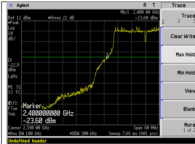
2422MHz_40MHz_n-mode_Lower Band Edge_Ant A
