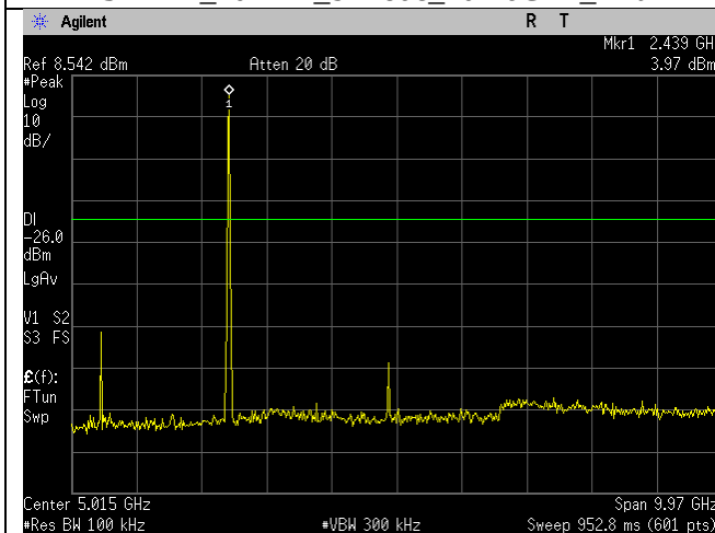
2437MHz_20MHz_b-mode_30MHz-10GHz_Ant A
