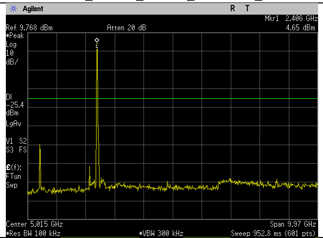
2412MHz_20MHz_n-mode_30MHz-10GHz_Ant B
