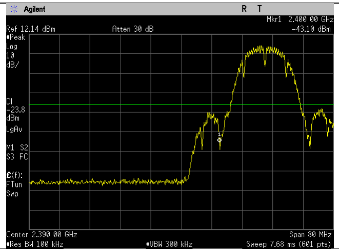
2412MHz_20MHz_b-mode_Lower Band Edge_Ant B
