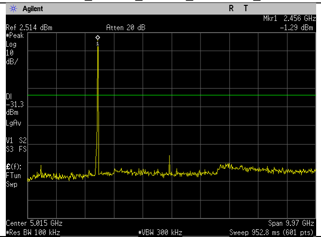
2462MHz_20MHz_b-mode_30MHz-10GHz_Ant B
