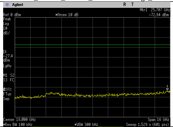
2422MHz_40MHz_n-mode_10-26GHz_Ant B
