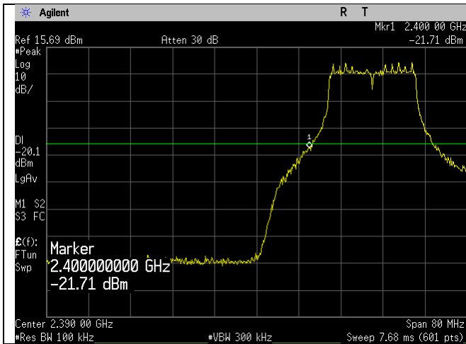
2412MHz_20MHz_g-mode_Lower Band Edge_Ant A
