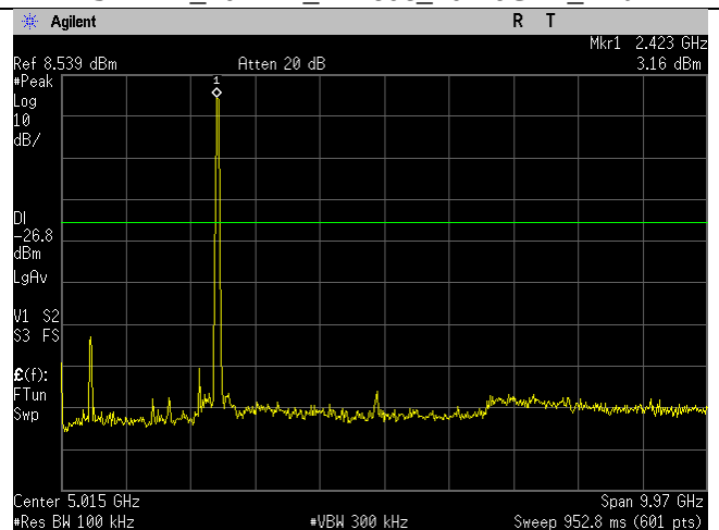
2437MHz_40MHz_n-mode_30MHz-10GHz_Ant B
