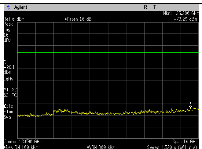
2452MHz_40MHz_n-mode_10-26GHz_Ant B
