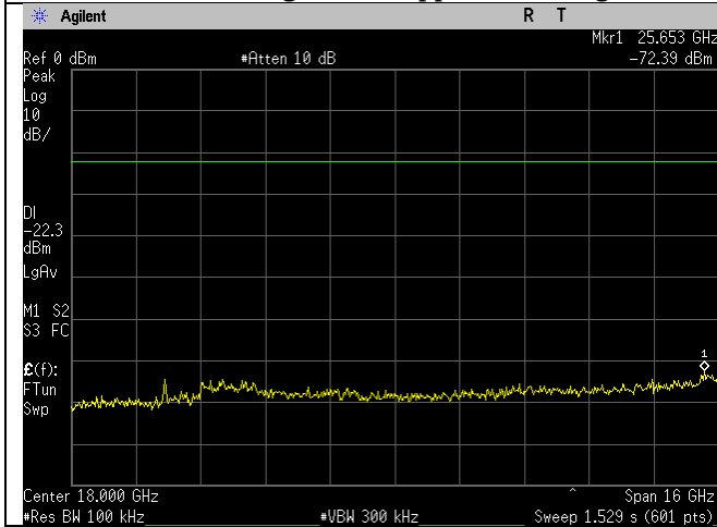
2462MHz_20MHz_n-mode_10-26GHz_Ant A
