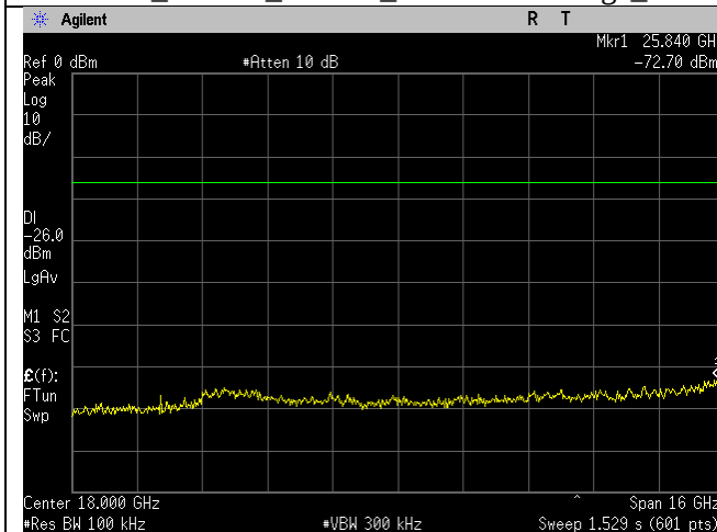
2437MHz_20MHz_b-mode_10-26GHz_Ant A
