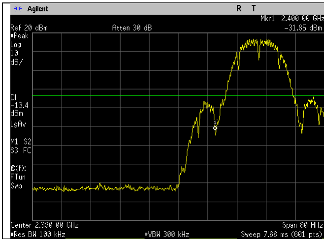
2412MHz_20MHz_b-mode_Lower Band Edge_Ant A
