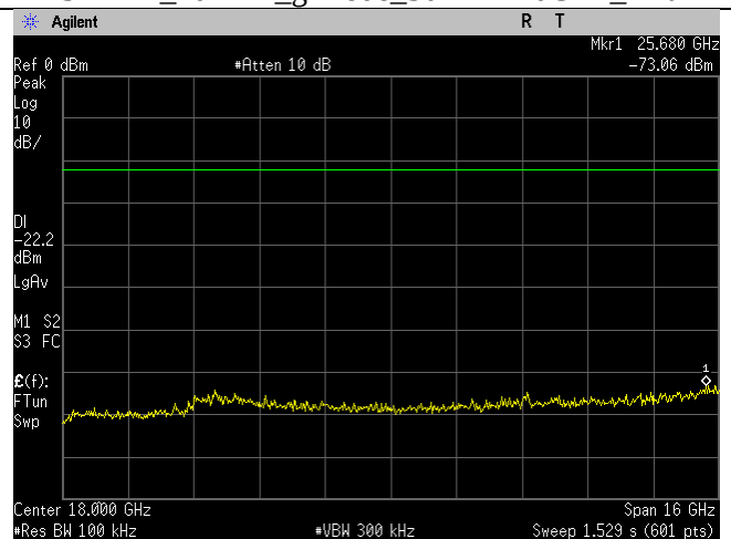
2437MHz_20MHz_n-mode_10-26GHz_Ant B
