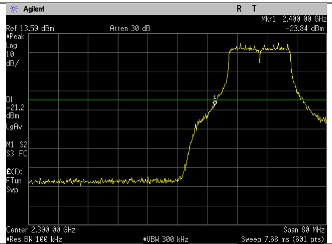
2412MHz_20MHz_g-mode_Lower Band Edge_Ant B
