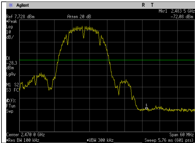
2462MHz_20MHz_b-mode_Upper Band Edge_Ant A
