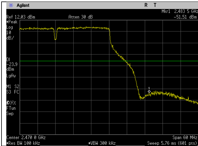
2452MHz_40MHz_n-mode_Upper Band Edge_Ant A
