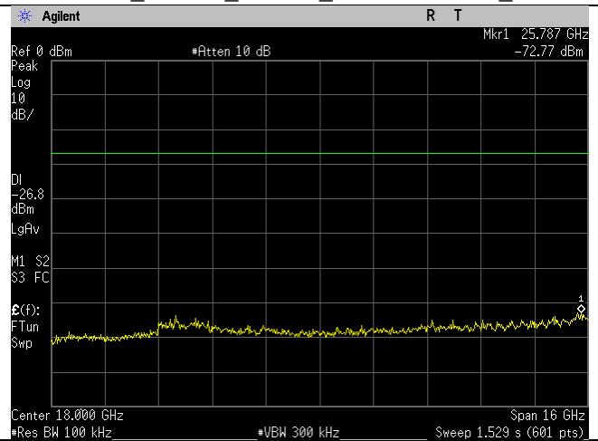
2437MHz_40MHz_n-mode_10-26GHz_Ant B
