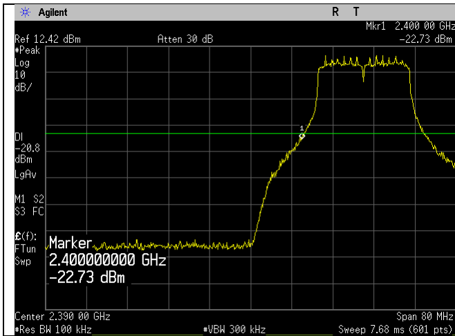
2412MHz_20MHz_n-mode_Lower Band Edge_Ant A
