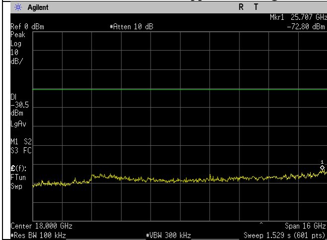
2462MHz_20MHz_b-mode_10-26GHz_Ant A
