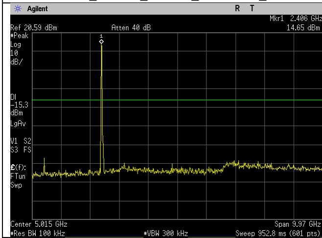
2412MHz_20MHz_b-mode_30MHz-10GHz_Ant A
