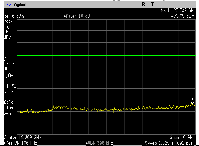
2462MHz_20MHz_b-mode_10-26GHz_Ant B
