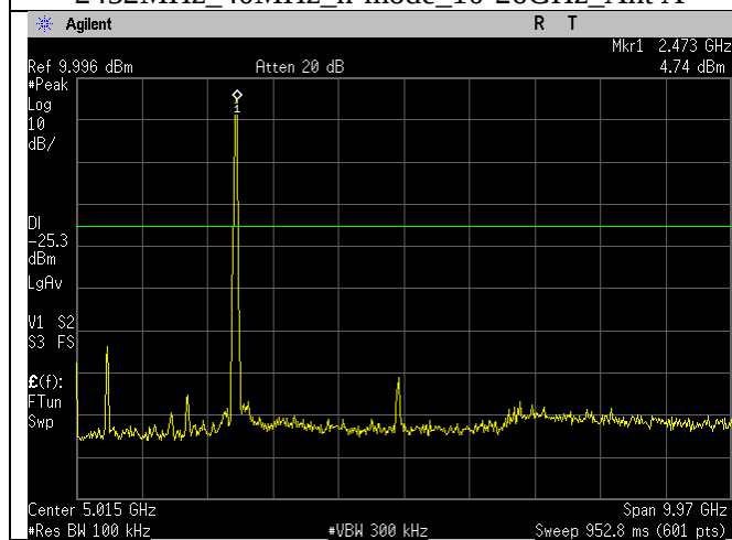
2452MHz_40MHz_n-mode_30MHz-10GHz_Ant A
