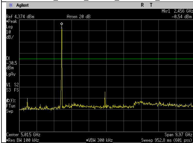
2462MHz_20MHz_b-mode_30MHz-10GHz_Ant A
