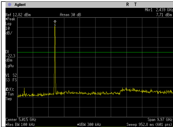
2437MHz_20MHz_n-mode_30MHz-10GHz_Ant A
