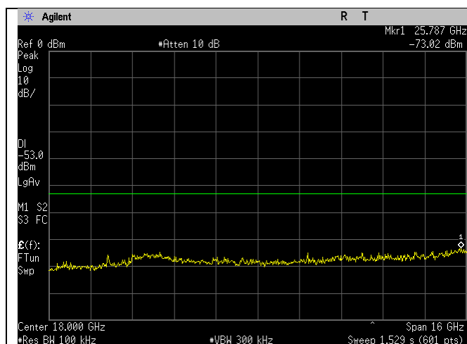
2452MHz_40MHz_n-mode_10-26GHz_Ant A
