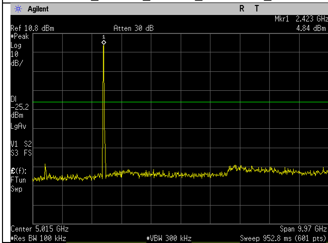
2412MHz_20MHz_n-mode_30MHz-10GHz_Ant A
