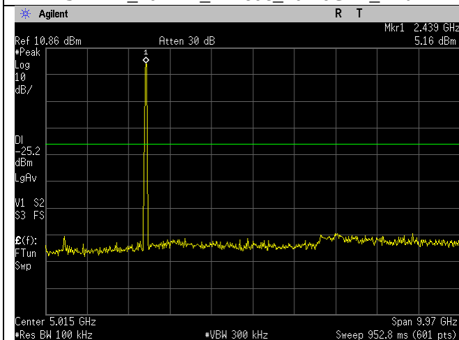
2437MHz_40MHz_n-mode_30MHz-10GHz_Ant A
