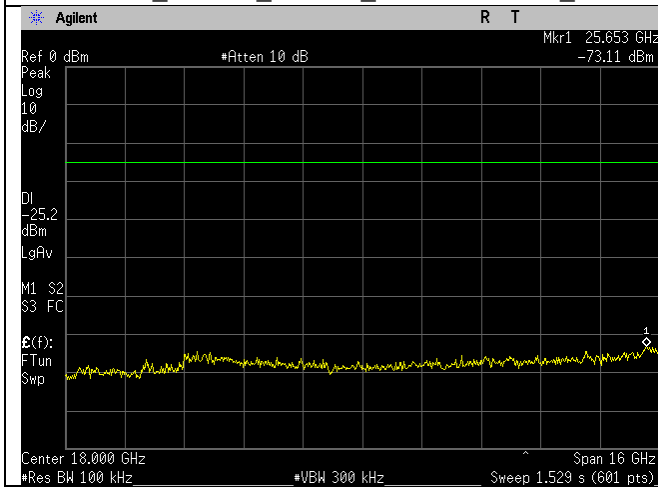
2437MHz_40MHz_n-mode_10-26GHz_Ant A
