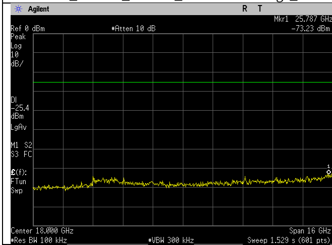
2422MHz_40MHz_n-mode_10-26GHz_Ant A
