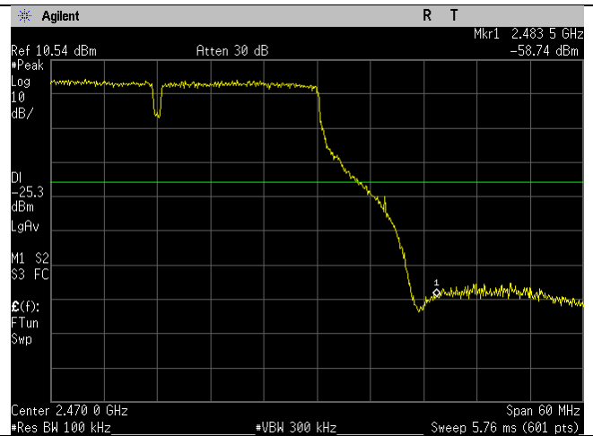
2452MHz_40MHz_n-mode_Upper Band Edge_Ant B
