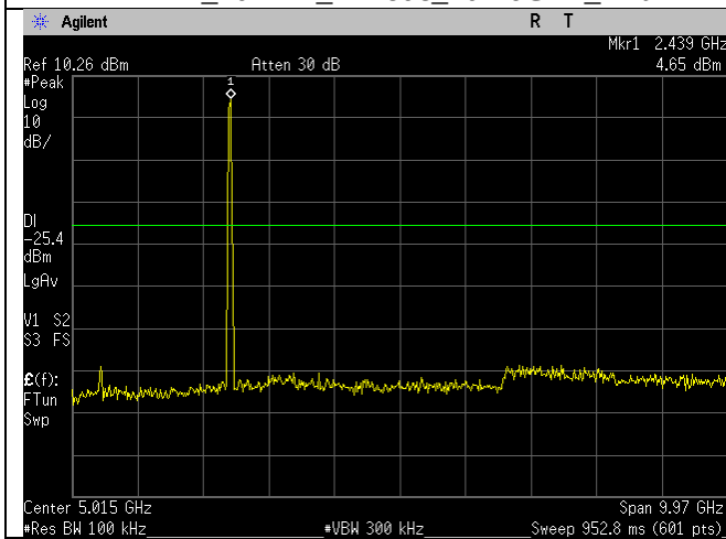
2422MHz_40MHz_n-mode_30MHz-10GHz_Ant A
