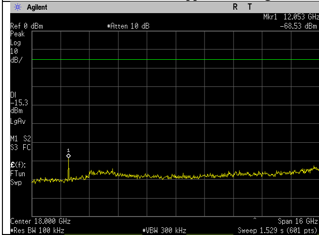
2412MHz_20MHz_b-mode_10-26GHz_Ant A
