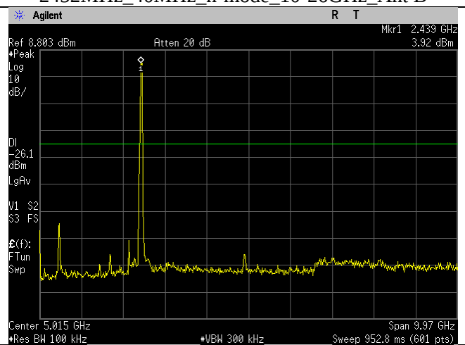
2452MHz_40MHz_n-mode_30MHz-10GHz_Ant B
