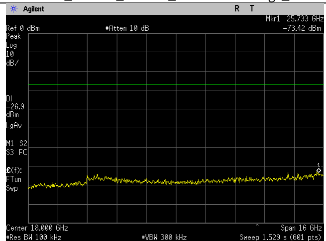
2437MHz_20MHz_b-mode_10-26GHz_Ant B
