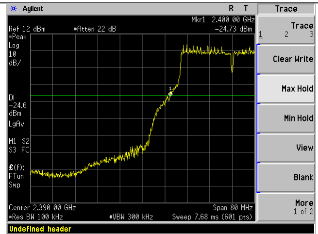
2422MHz_40MHz_n-mode_Lower Band Edge_Ant B
