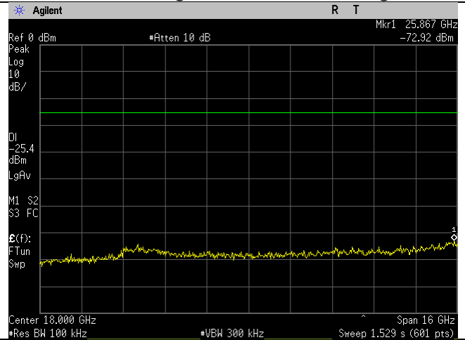
2412MHz_20MHz_n-mode_10-26GHz_Ant B
