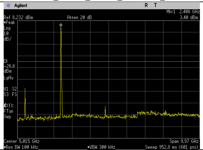
2412MHz_20MHz_b-mode_30MHz-10GHz_Ant B
