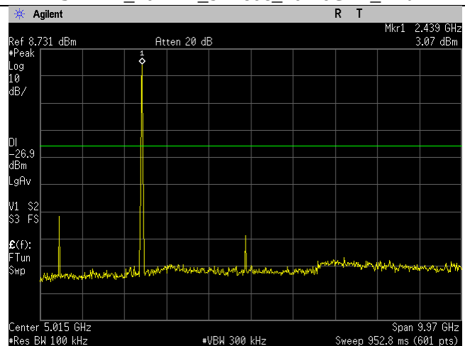
2437MHz_20MHz_b-mode_30MHz-10GHz_Ant B
