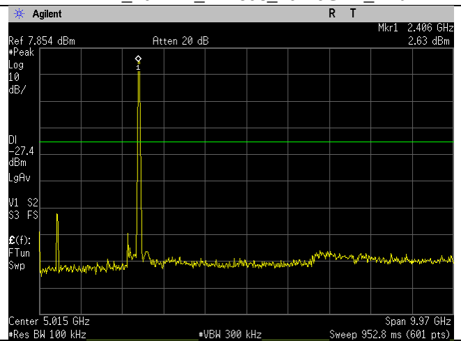
2422MHz_40MHz_n-mode_30MHz-10GHz_Ant B
