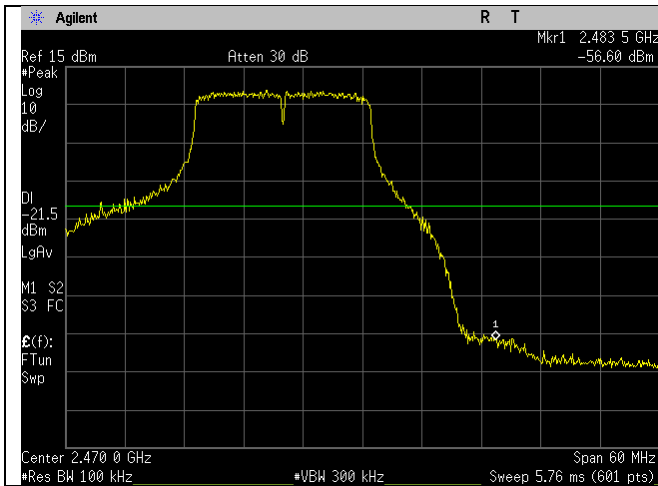
2462MHz_20MHz_n-mode_Upper Band Edge_Ant A
