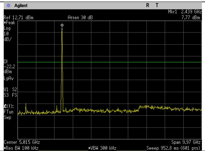
2437MHz_20MHz_n-mode_30MHz-10GHz_Ant B
