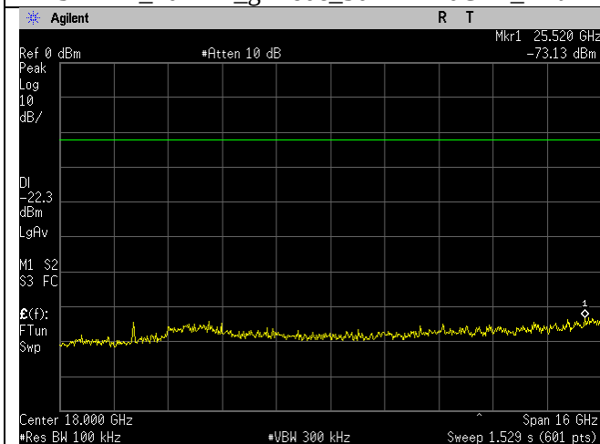
2437MHz_20MHz_n-mode_10-26GHz_Ant A
