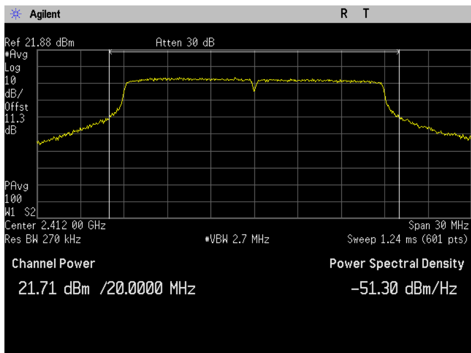
WIFI_Low Ch_2412MHz_20MHz BW_n-mode_Output Power_Port 1
