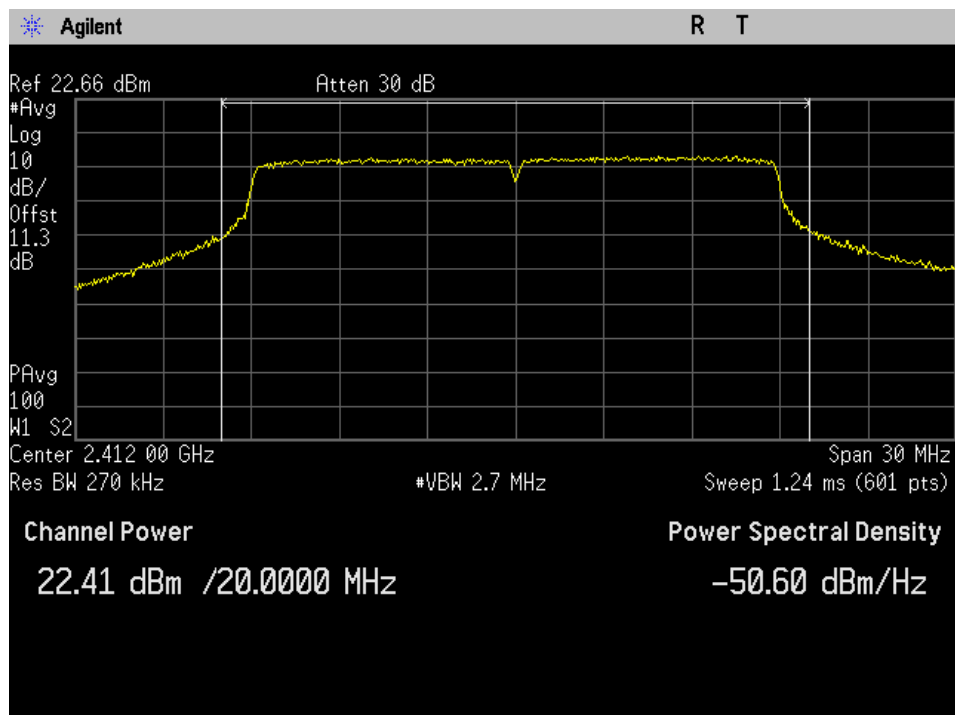
WIFI_Low Ch_2412MHz_20MHz BW_n-mode_Output Power_Port 2
