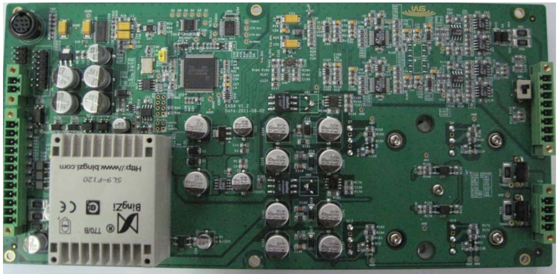
(1) EUT Photo
