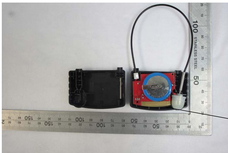
TX&RX ANTENNA
