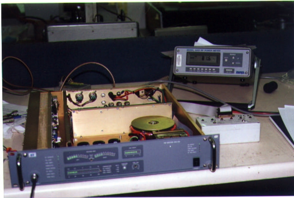
100W stereo transmitter connected to the test equipment on the bench showing output power.
