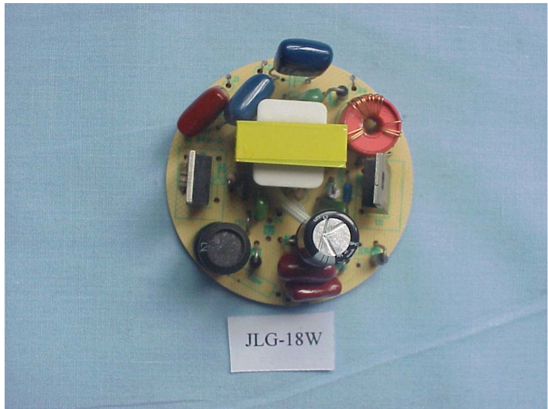
FIGURE 2 ENERGY SAVING LAMP (M/N: JLG-18W) MAIN BOARD (COMPONENT SIDE)
