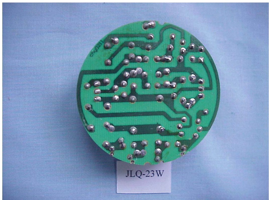
FIGURE 21 ENERGY SAVING LAMP (M/N: JLQ-23W) MAIN BOARD (SOLDERED SIDE)
