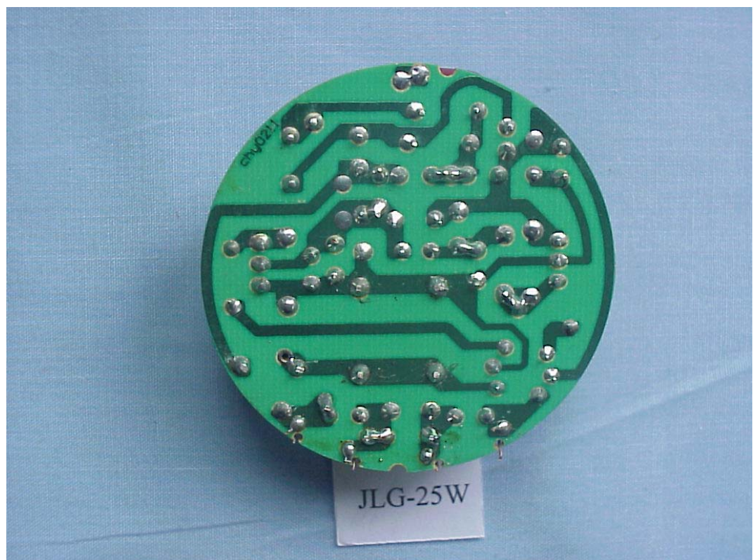
FIGURE 12 ENERGY SAVING LAMP (M/N: JLG-25W) MAIN BOARD (SOLDERED SIDE)
