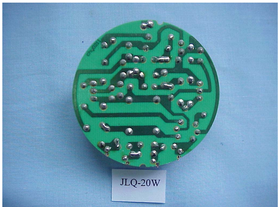
FIGURE 18 ENERGY SAVING LAMP (M/N: JLQ-20W) MAIN BOARD (SOLDERED SIDE)
