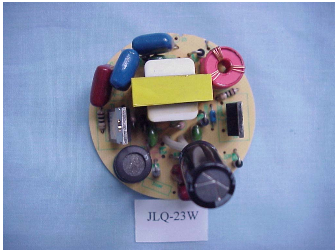
FIGURE 20 ENERGY SAVING LAMP (M/N: JLQ-23W) MAIN BOARD (COMPONENT SIDE)
