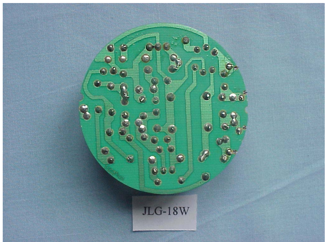
FIGURE 3 ENERGY SAVING LAMP (M/N: JLG-18W) MAIN BOARD (SOLDERED SIDE)
