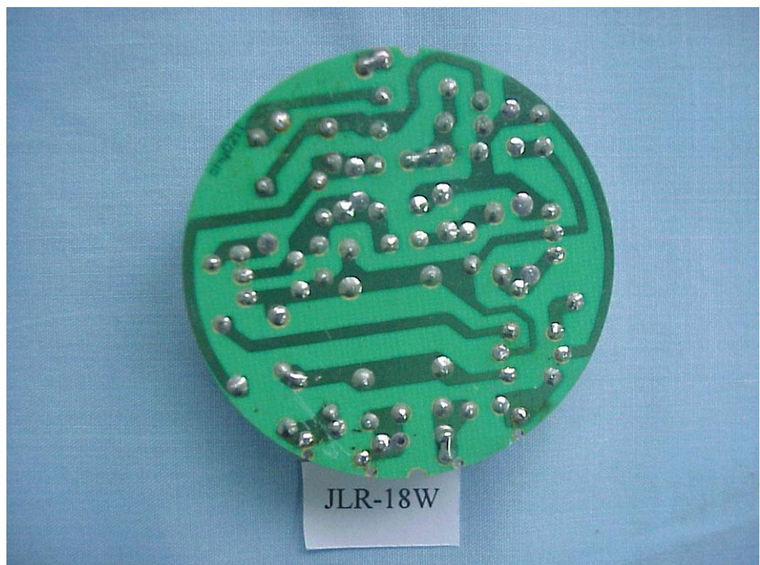
FIGURE 27 ENERGY SAVING LAMP (M/N: JLR-18W) MAIN BOARD (SOLDERED SIDE)
