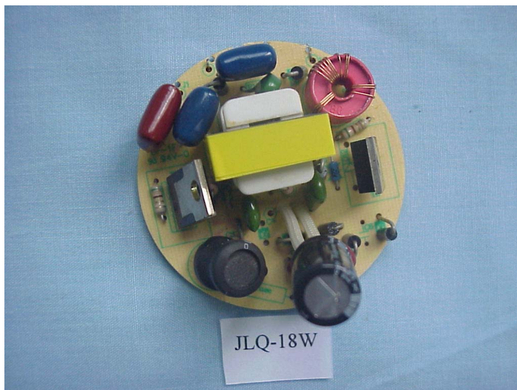
FIGURE 14 ENERGY SAVING LAMP (M/N: JLQ-18W) MAIN BOARD (COMPONENT SIDE)
