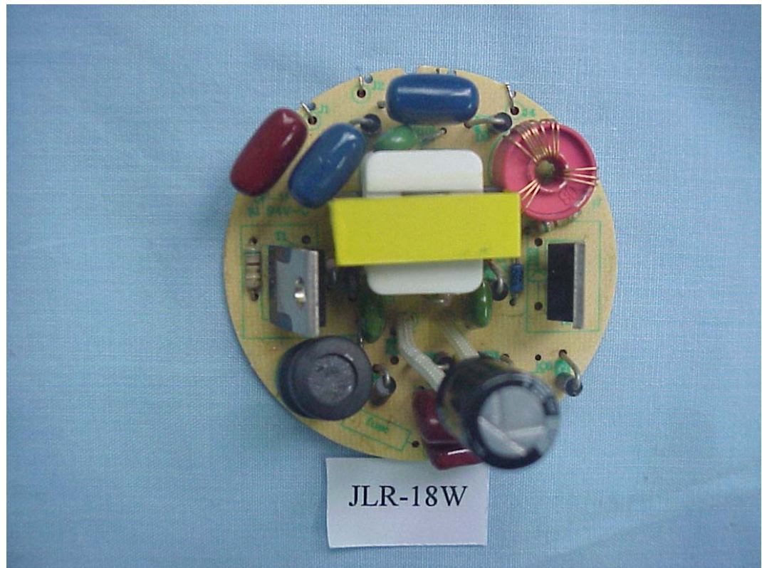
FIGURE 26 ENERGY SAVING LAMP (M/N: JLR-18W) MAIN BOARD (COMPONENT SIDE)
