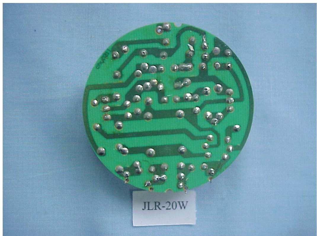
FIGURE 30 ENERGY SAVING LAMP (M/N: JLR-20W) MAIN BOARD (SOLDERED SIDE)
