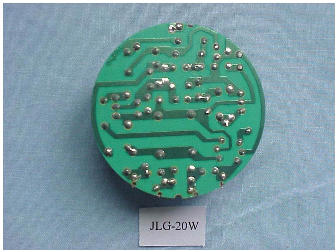
FIGURE 6 ENERGY SAVING LAMP (M/N: JLG-20W) MAIN BOARD (SOLDERED SIDE)
