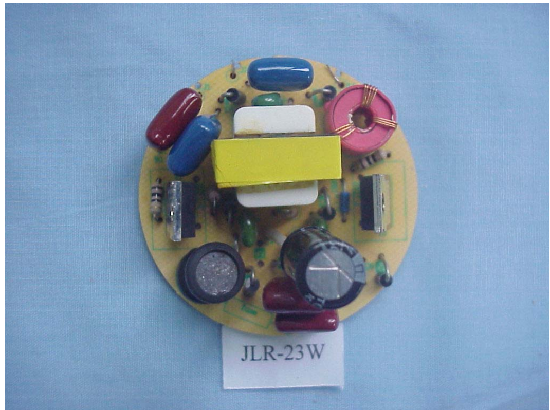
FIGURE 32 ENERGY SAVING LAMP (M/N: JLR-23W) MAIN BOARD (COMPONENT SIDE)
