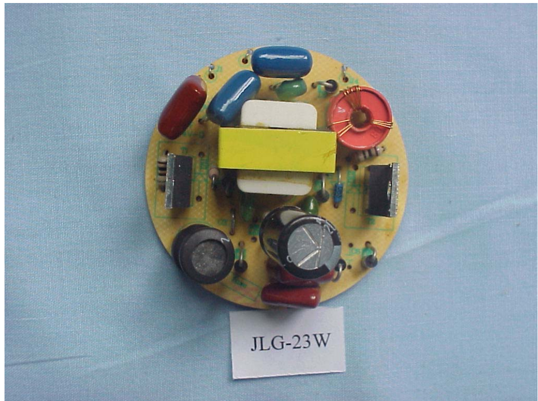
FIGURE 8 ENERGY SAVING LAMP (M/N: JLG-23W) MAIN BOARD (COMPONENT SIDE)
