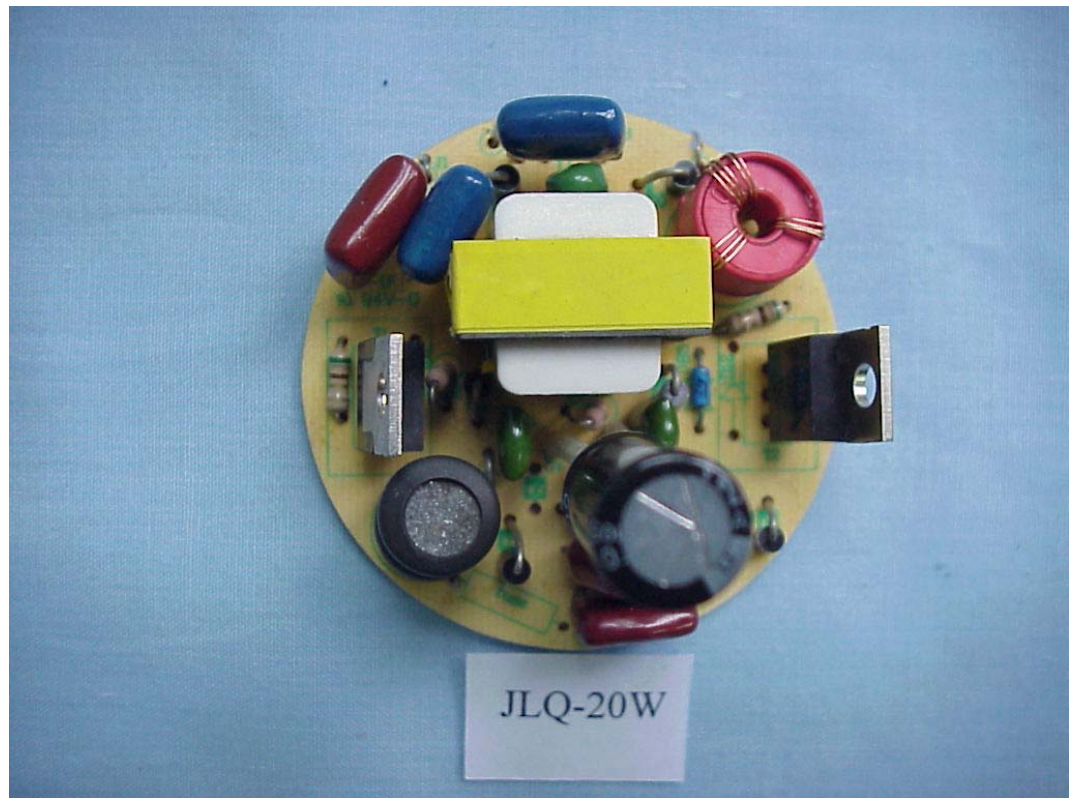
FIGURE 17 ENERGY SAVING LAMP (M/N: JLQ-20W) MAIN BOARD (COMPONENT SIDE)
