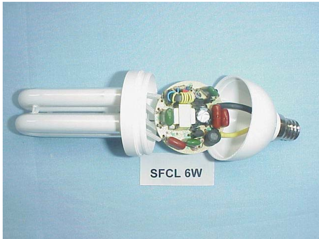
FIGURE 10 ENERGY SAVING LAMP (M/N: SFCL-6W) COVER REMOVED
