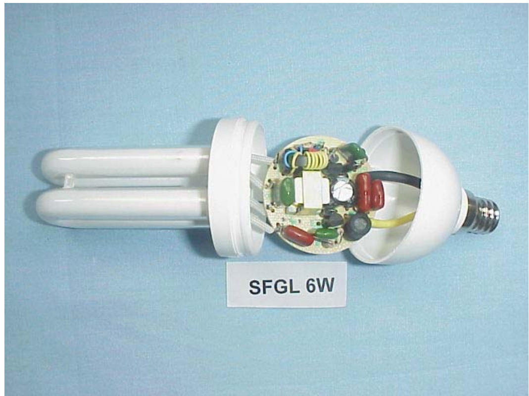
FIGURE 16 ENERGY SAVING LAMP (M/N: SFGL-6W) COVER REMOVED
