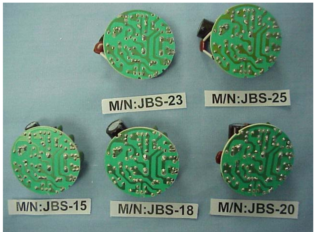
FIGURE 6 ELECTRONIC ENERGY SAVING LAMP (M/N: JBS SERIES) MAIN BOARD (SOLDERED SIDE)
