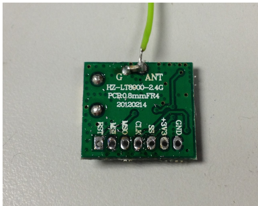
Internal View (Transmitter)
