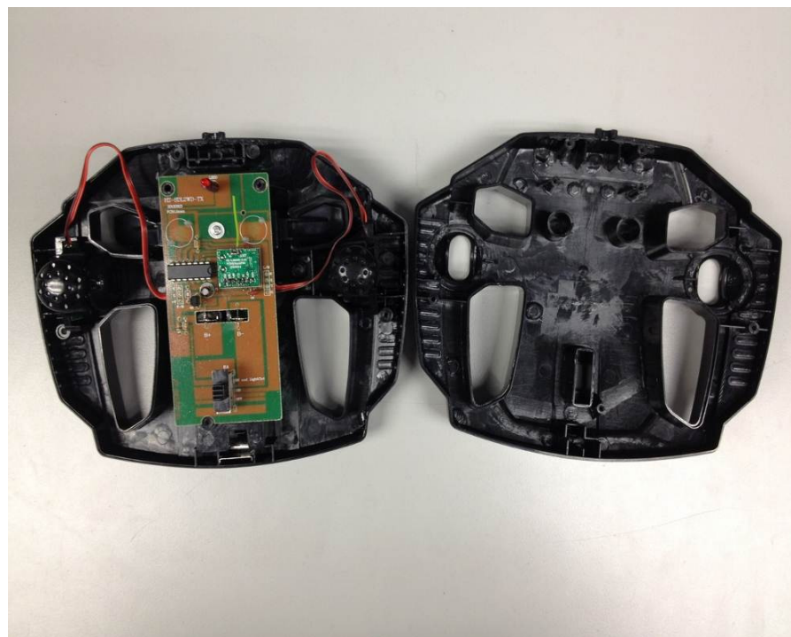
Internal View (Transmitter)
