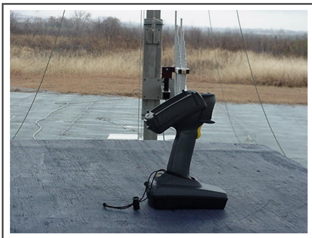
Radiated Emissions – Side View
