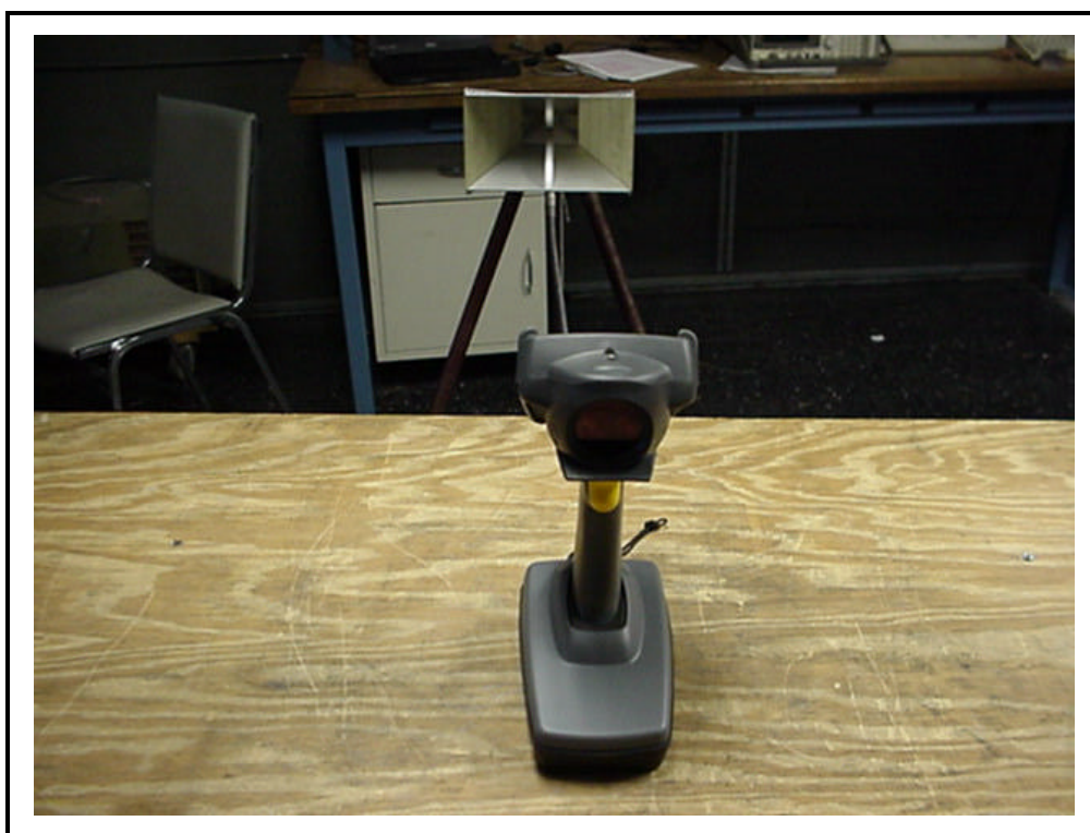
Microwave Radiated Emissions – Back View
