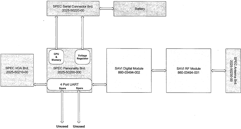
STR7200 MODULE BLOCK DIAGRAM 2025-50100-000
