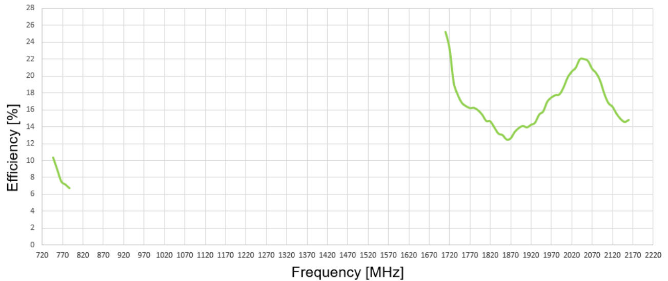
Figure 1; Antenna Efficiency from 746MHz to 2160 MHz
