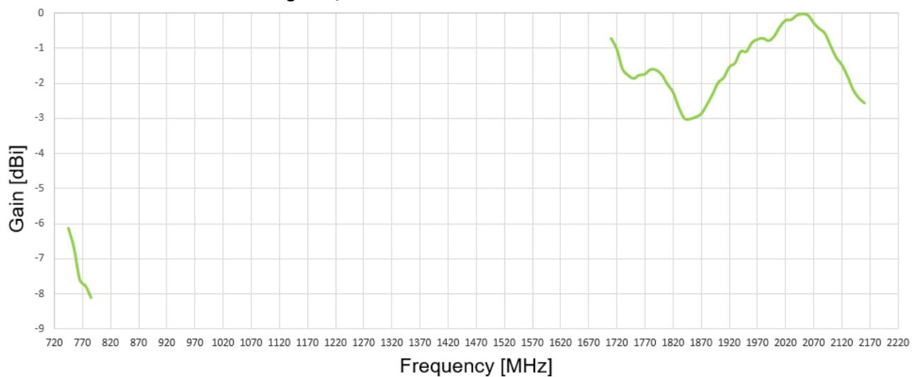
Figure 2; Antenna Peak Gain from 746MHz to 2160 MHz
