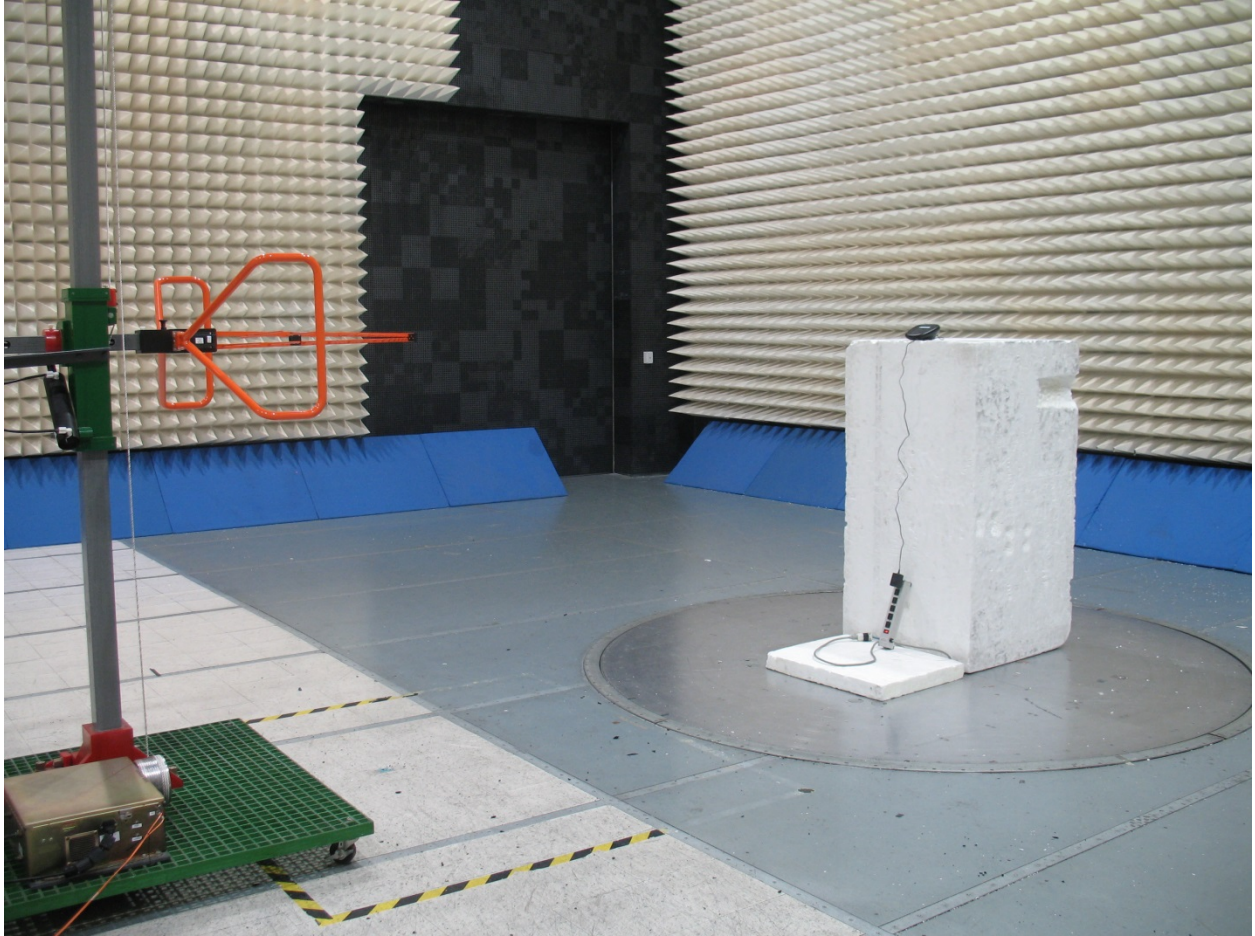
Setup – Intentional emissions, 30MHz-1GHz
