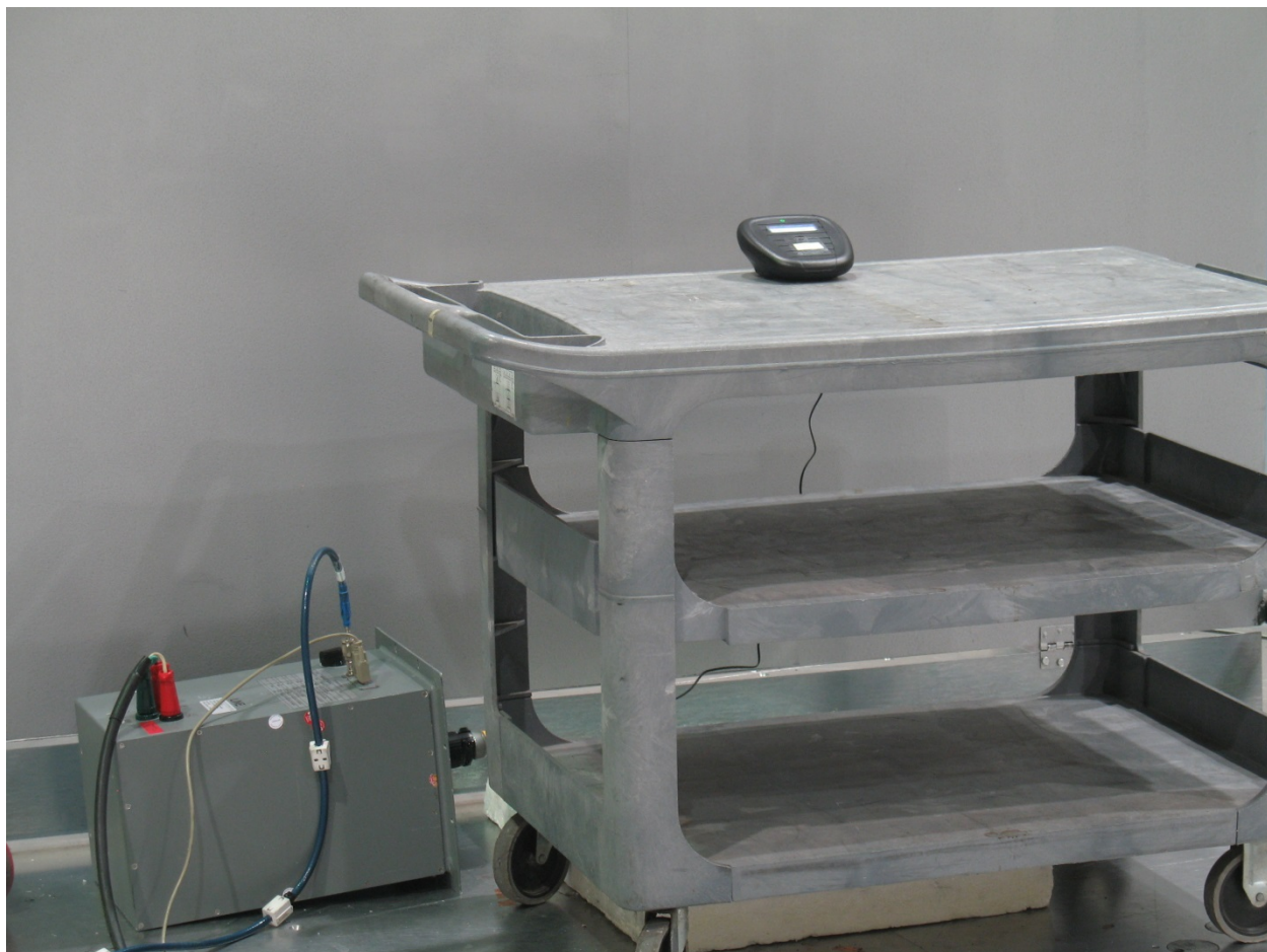
Setup – Conducted emissions
