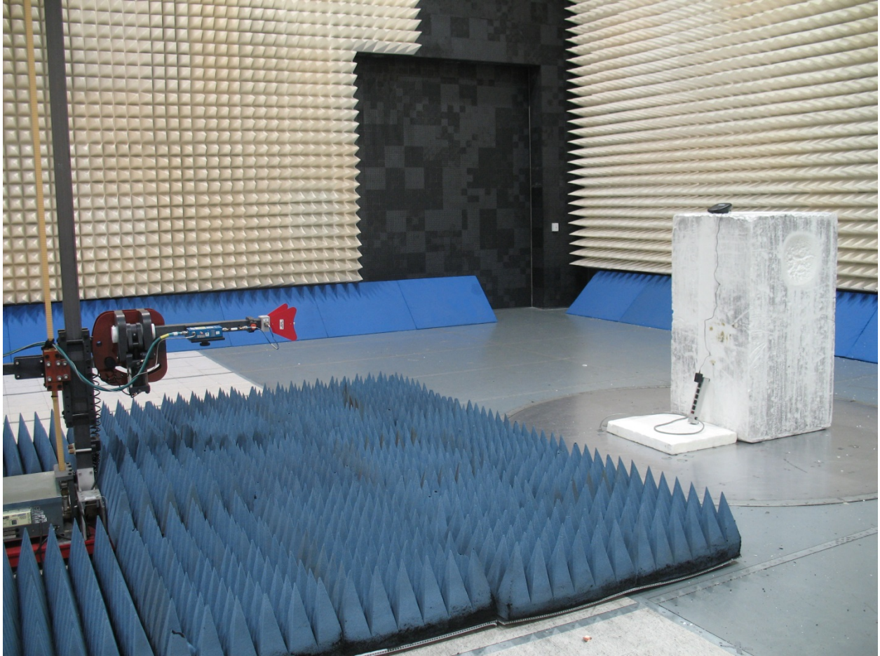
Setup – Intentional emissions, > 1GHz
