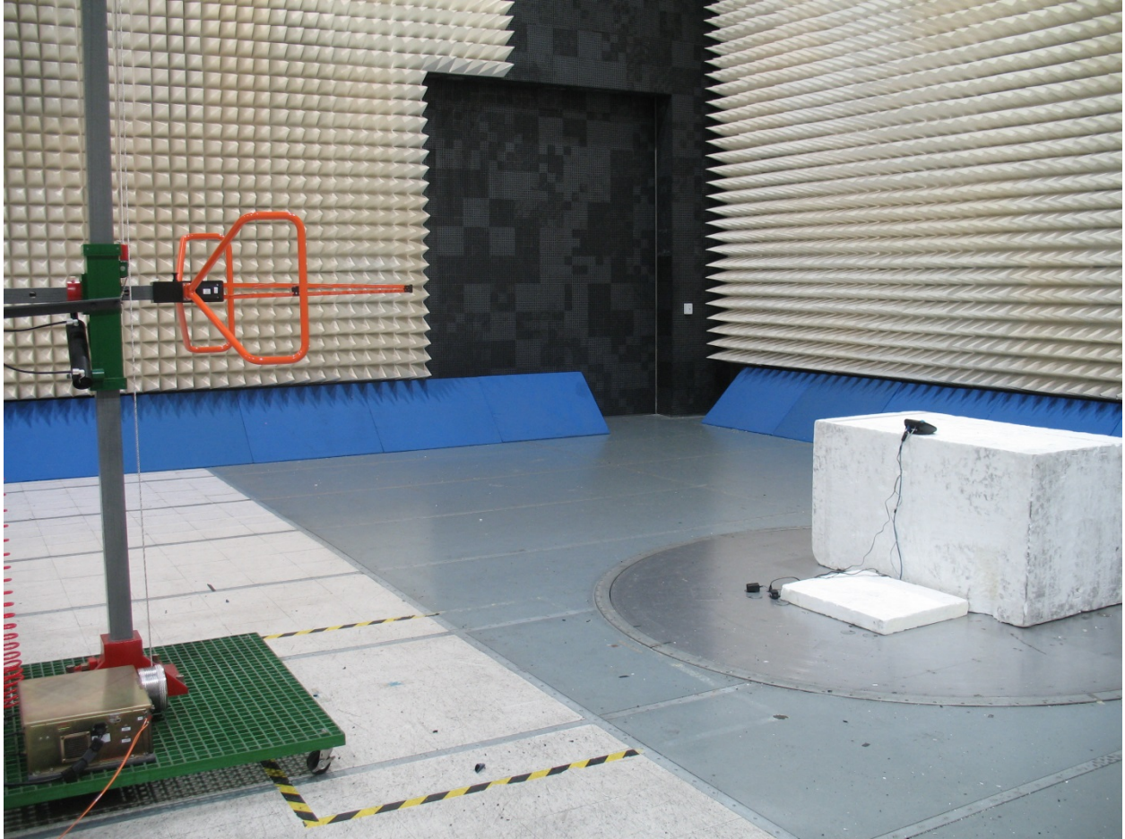
Setup – Unintentional emissions, 30MHz-1GHz
