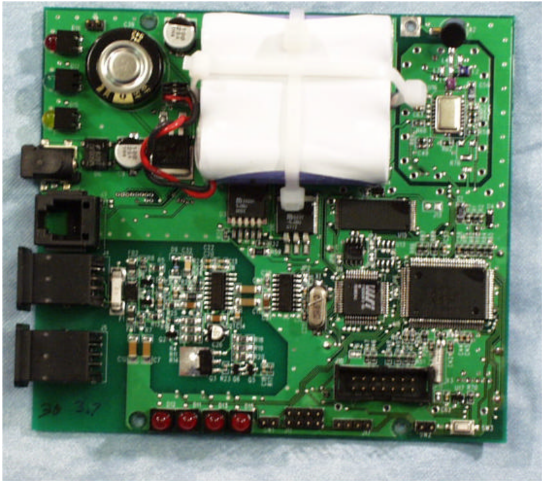
TOP OF BOARD
