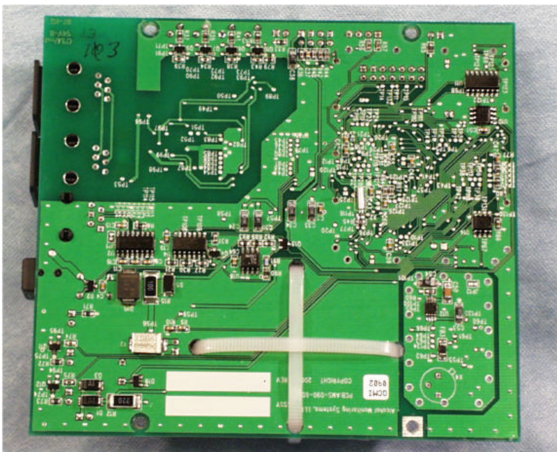
BACK OF BOARD
