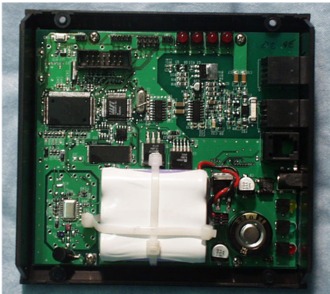
INSIDE BOARD MOUNTED
