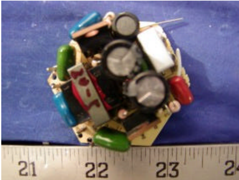
EUT - Component View (SPW-20E)
