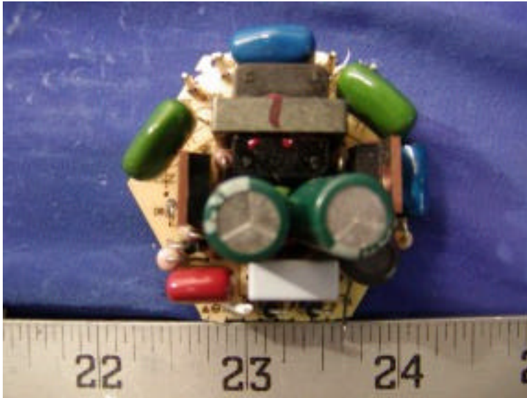
EUT - Component View (SPW-26E)
