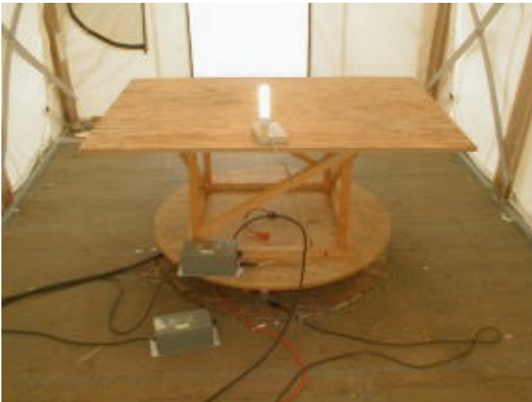
Conducted Emission Photograph – Rear View (REW-15E)
