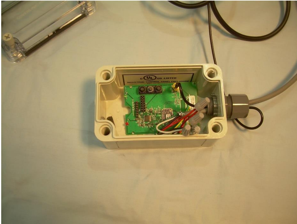
Photograph 5 – View of PCB in Housing
