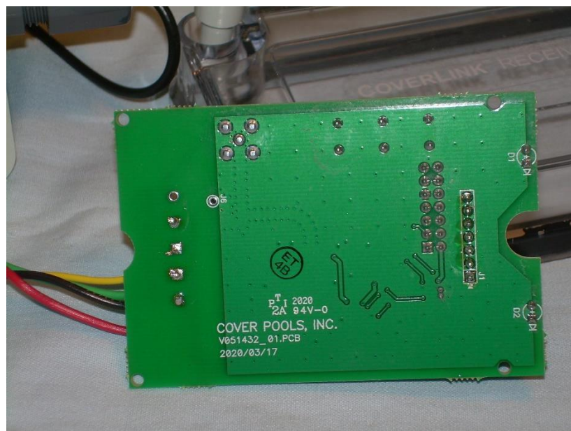
Photograph 12: Trace Side of the PCB
