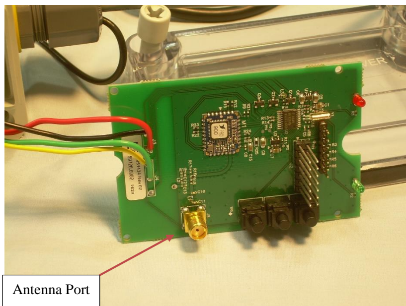
Photograph 11: Component Side of the PCB
