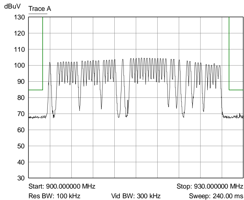
Graph 13: Emissions While Hopping
