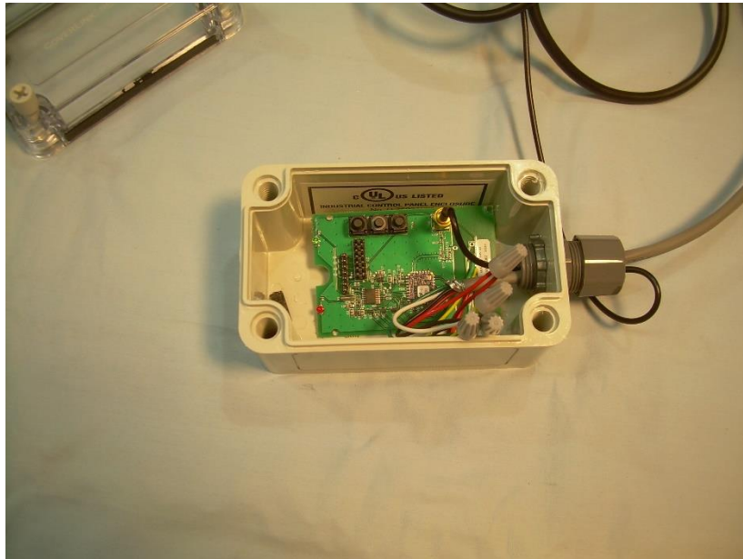
Photograph 10: View of the PCB in the Housing
