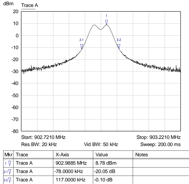
Graph 2: Lowest Channel 20 dB Bandwidth
