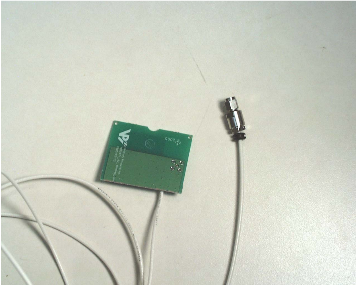
Trace Side of the Splat Antenna
