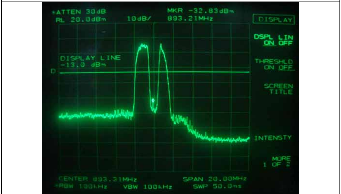
Downlink: IS-95 CDMA - High Channel
