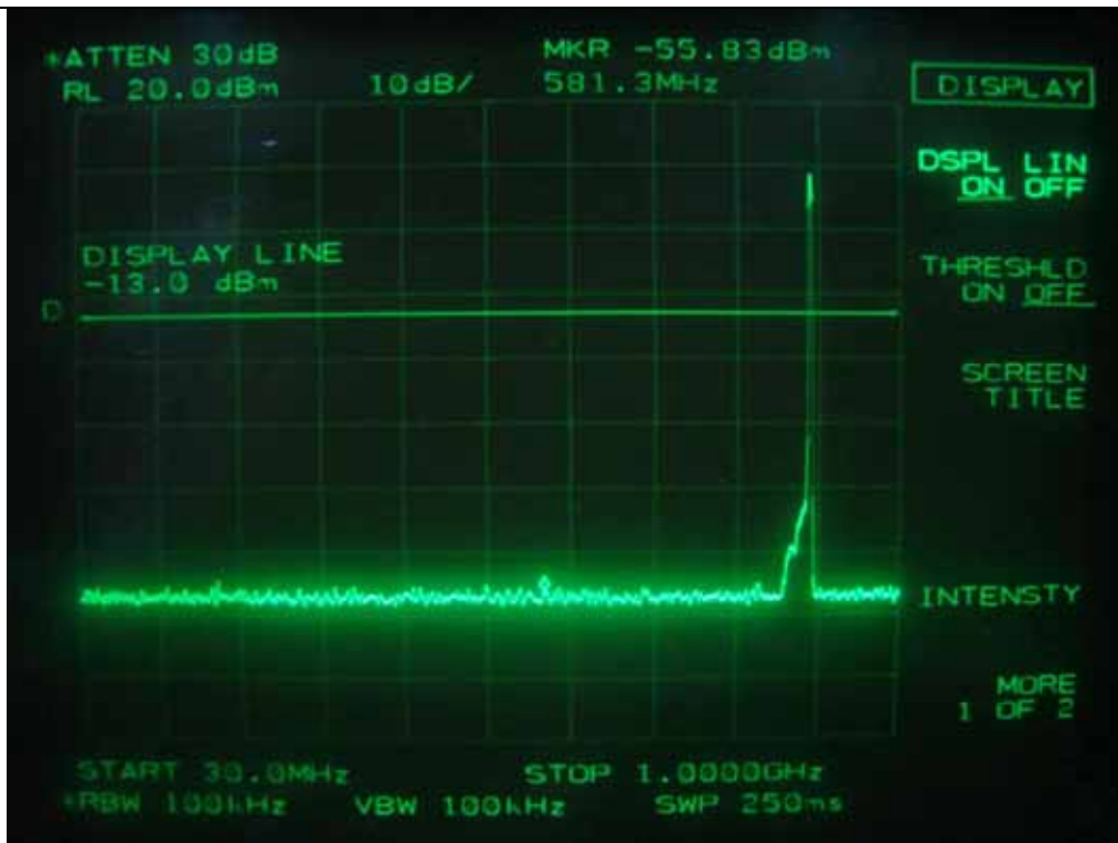
Downlink: 1xEVDO - High Channel
