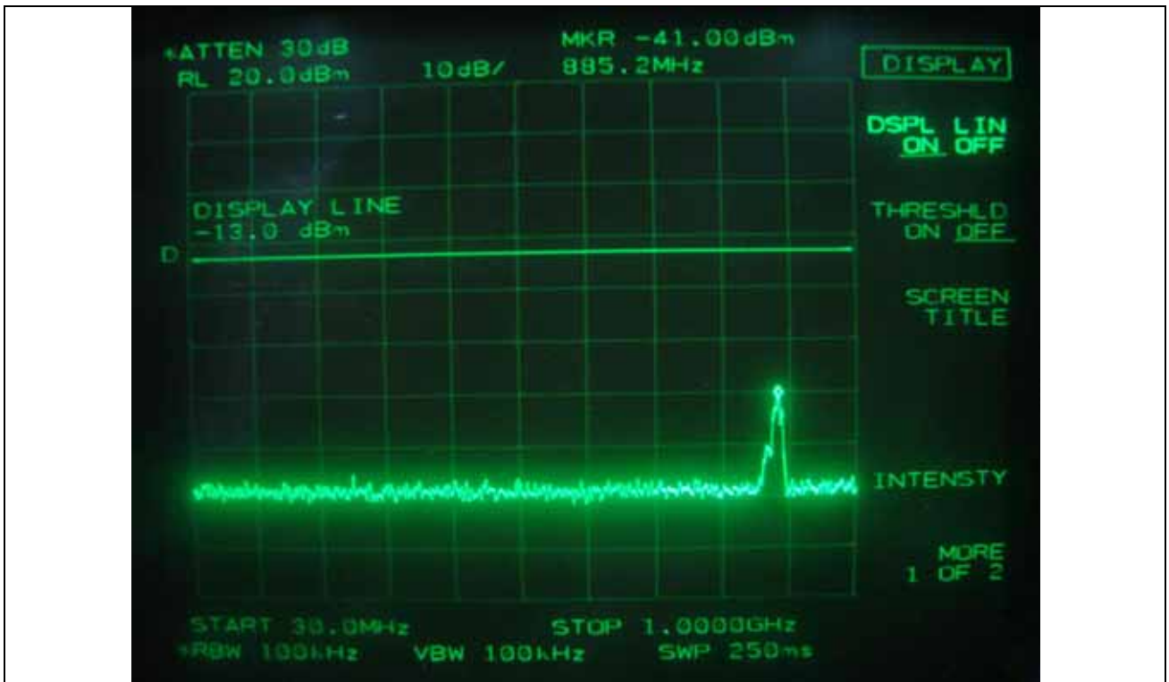
Downlink: 1xEVDO - Low Channel
