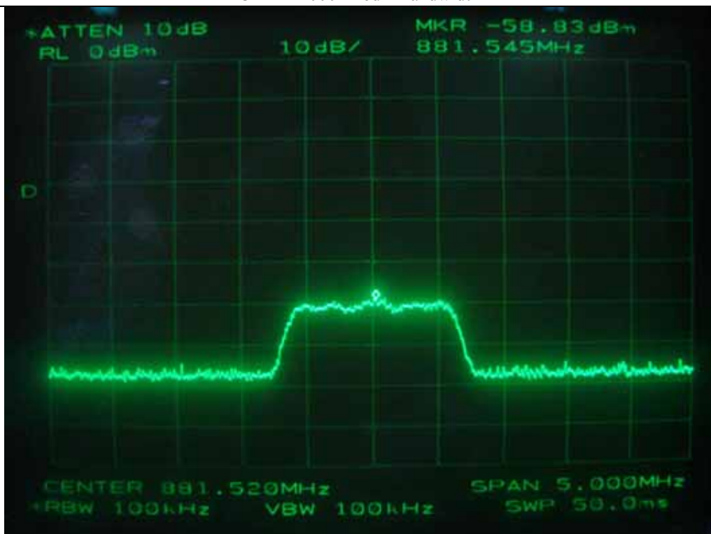
CDMA 2000 – Input Signal
