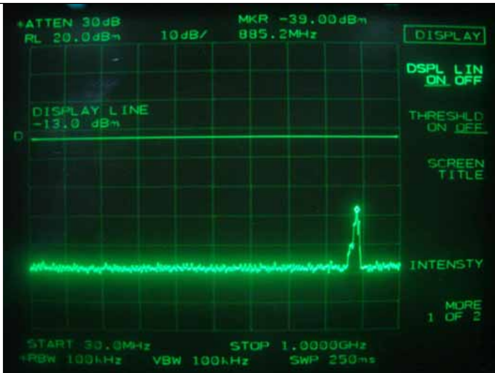
Downlink: 1xEVDO - Middle Channel
