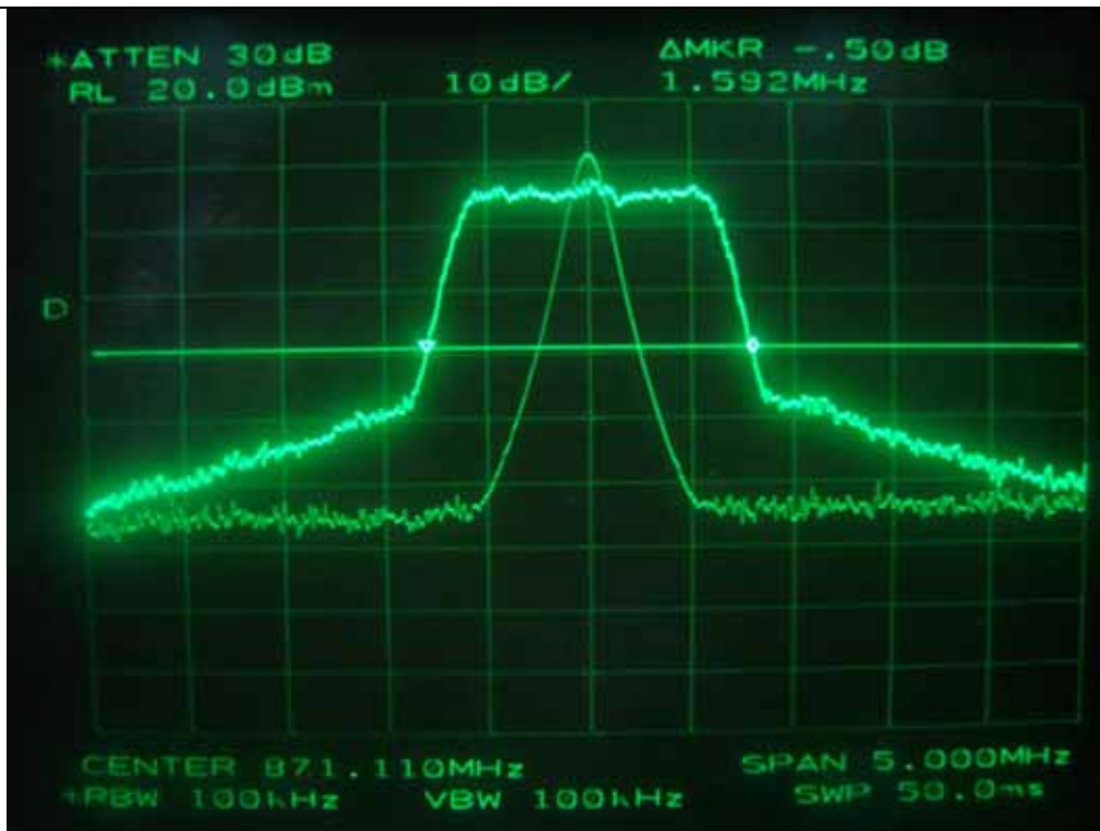
IS-95 CDMA - 26dB Bandwidth
