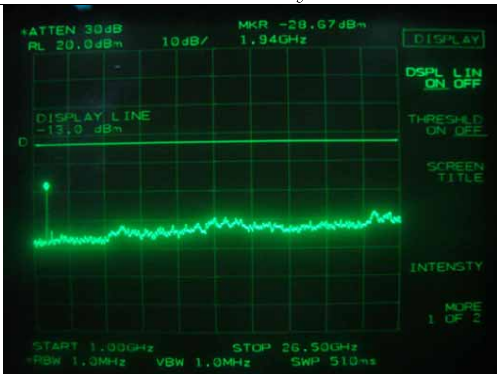
Downlink: CDMA 2000- High Channel
