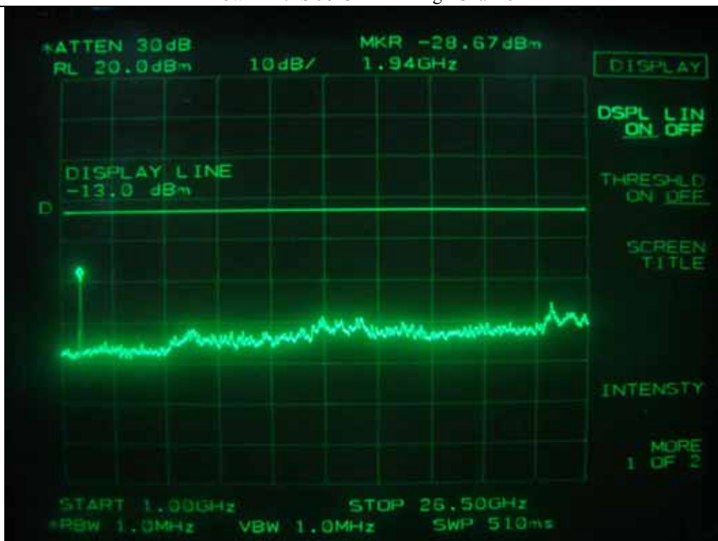
Downlink: IS-95 CDMA - High Channel
