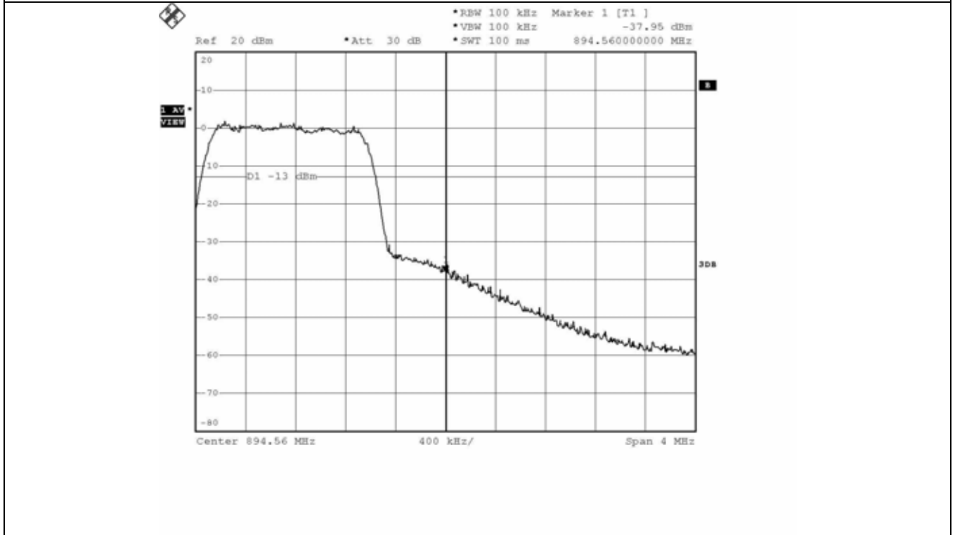
Downlink: IS-95 CDMA - Band Edge-High Channel
