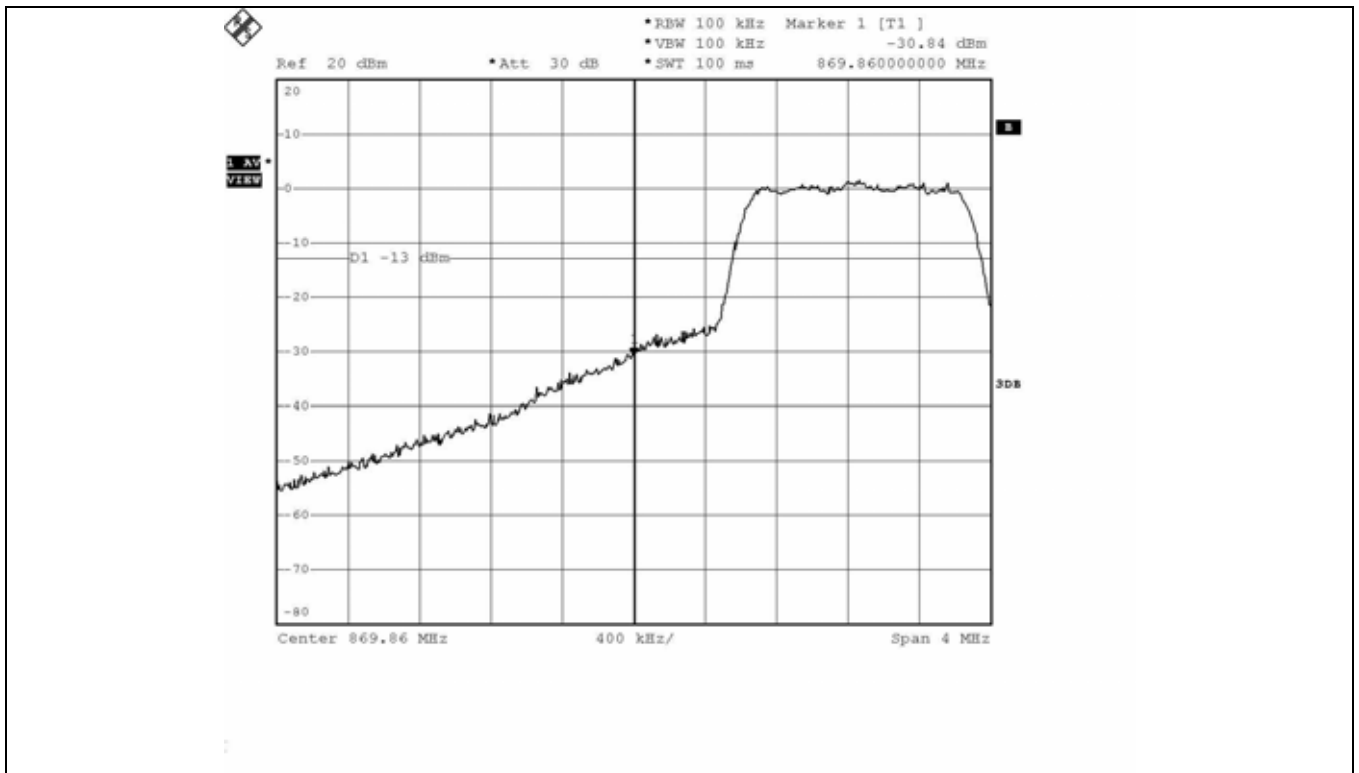
Downlink: IS-95 CDMA - Band Edge-Low Channel
