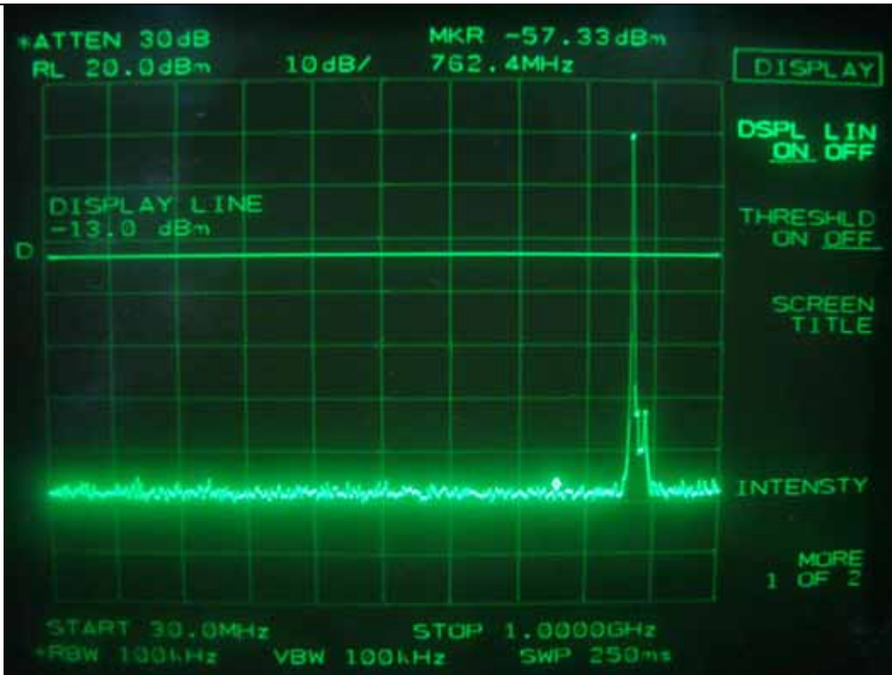
Downlink: 1xEVDO - Low Channel
