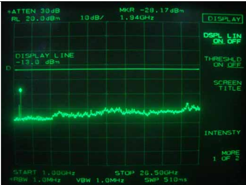
Downlink: CDMA 2000- Low Channel
