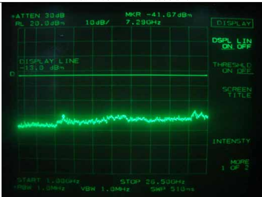
Downlink: CDMA 2000- Middle Channel
