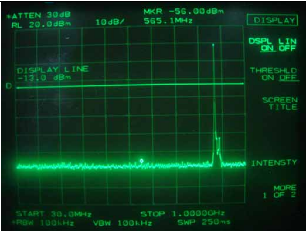
Downlink: IS-95 CDMA - Low Channel
