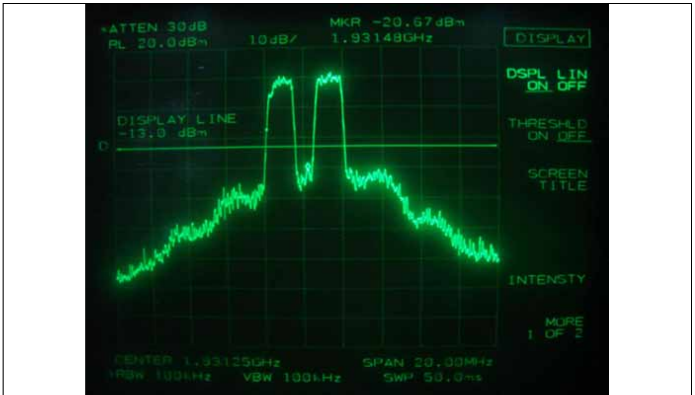
Downlink: IS-95 CDMA - Low Channel
