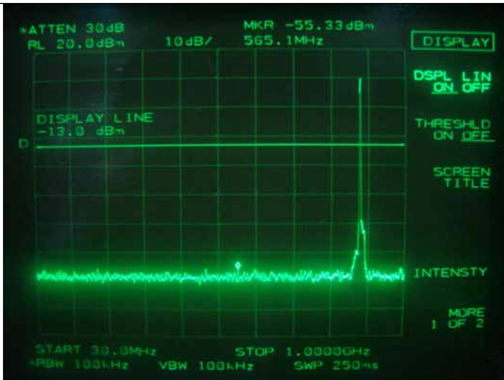
Downlink: IS-95 CDMA - Middle Channel
