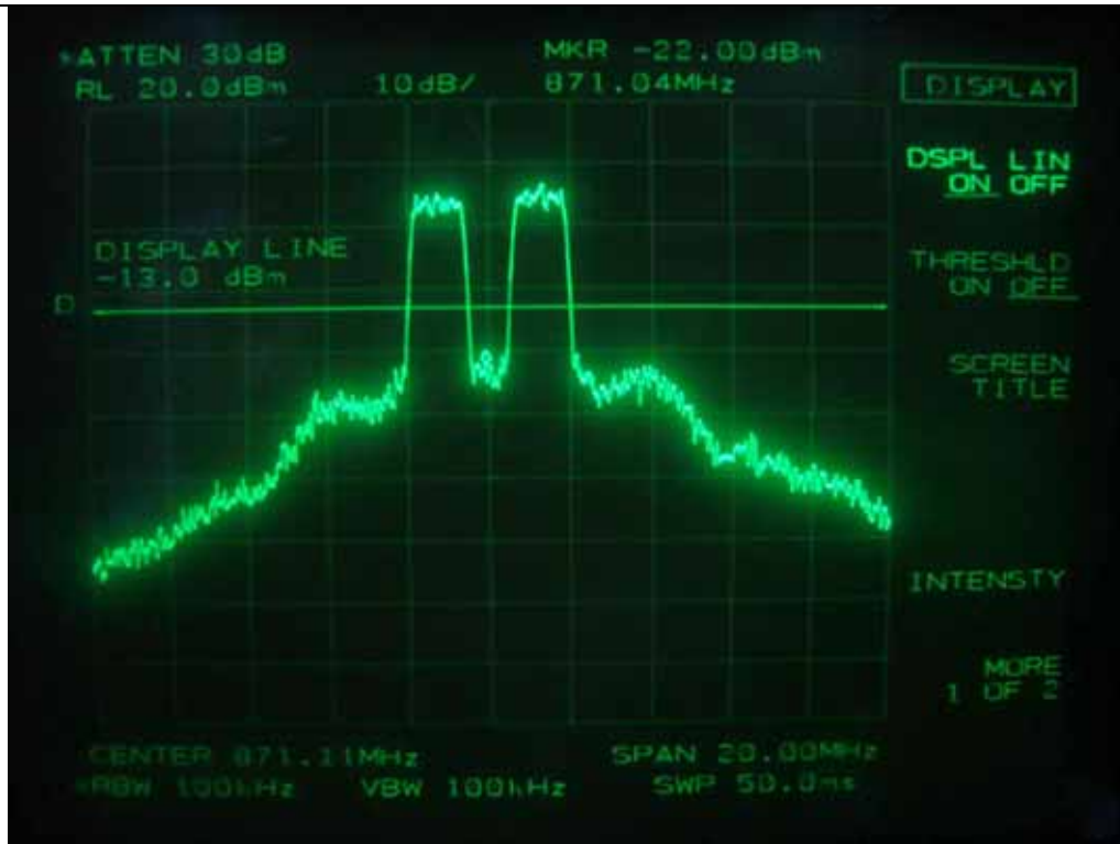
Downlink: 1xEVDO - Low Channel
