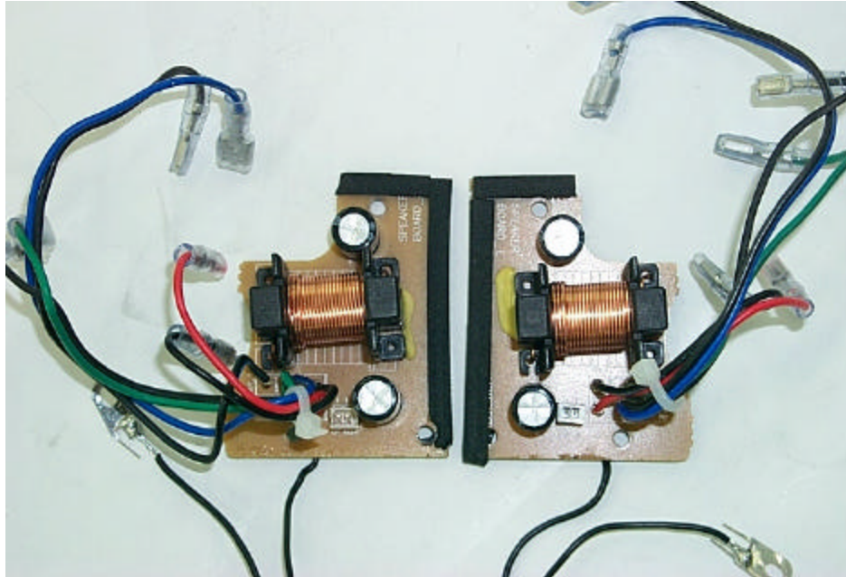
< Speaker Board(L/R) – Top View >
