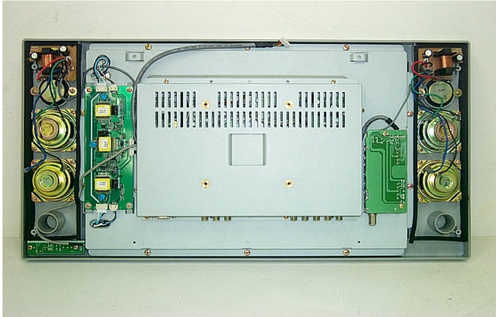
< Internal View – With Main Board Cover >
