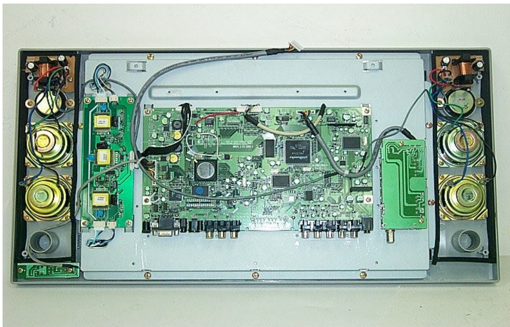
< Internal View - Without Main Board Cover >
