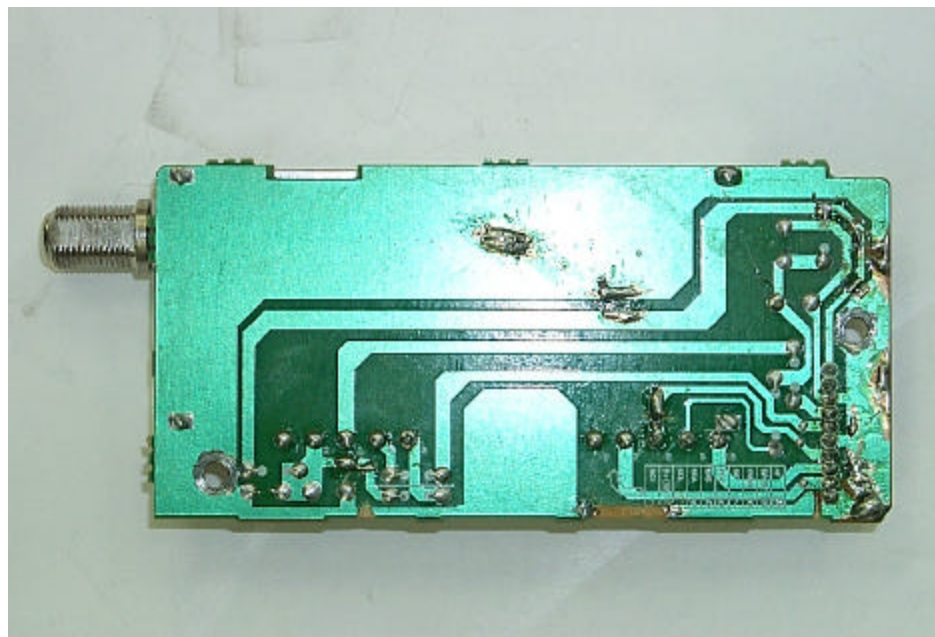
< Tuner Board – Bottom View >
