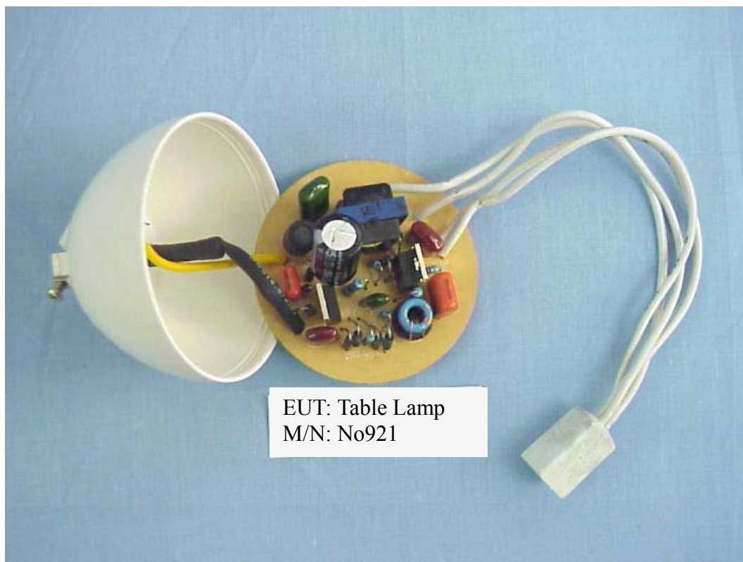
FIGURE 3 TABLE LAMP (M/N: No921) COVER REMOVED#2 (BALLAST M/N KFE-C22W)
