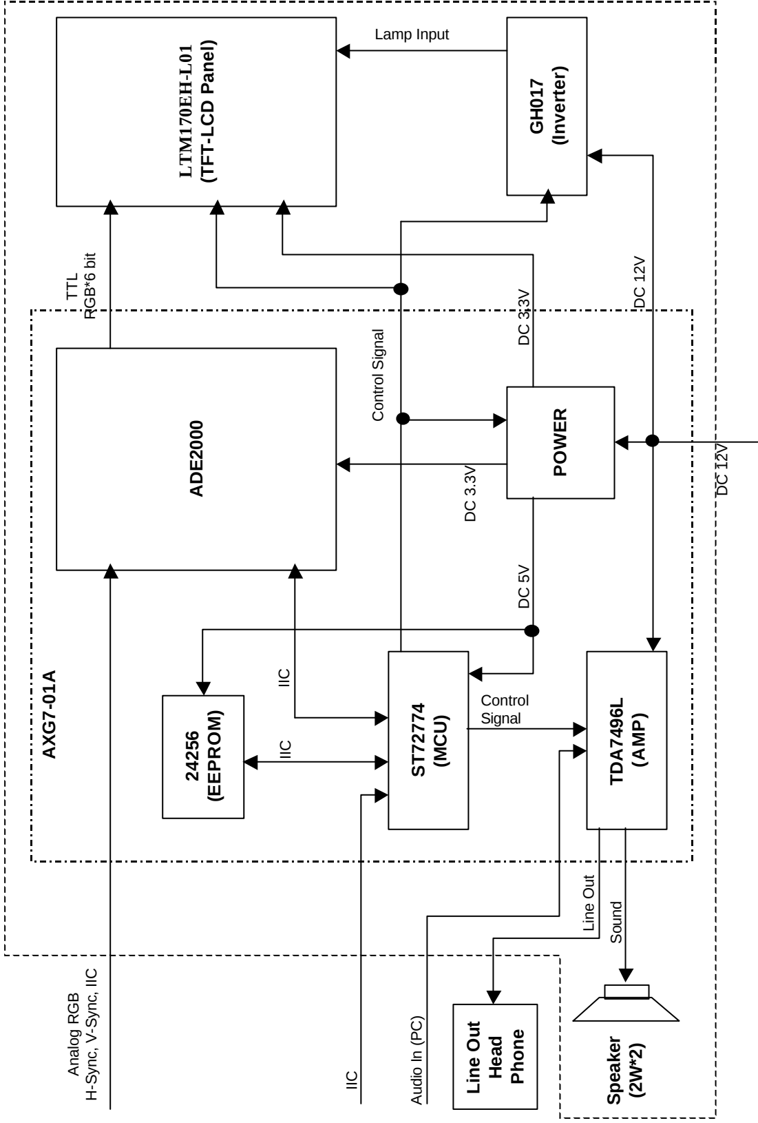
EN-7500 Monitor Block Diagram
