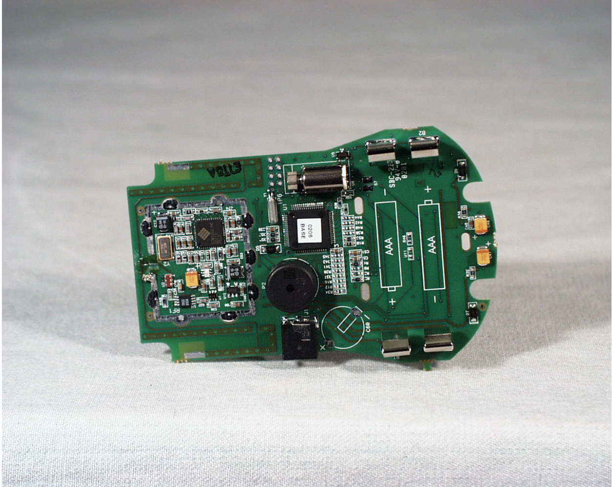
Bottom view of the FoolProof 1.0 PCB (Base)
