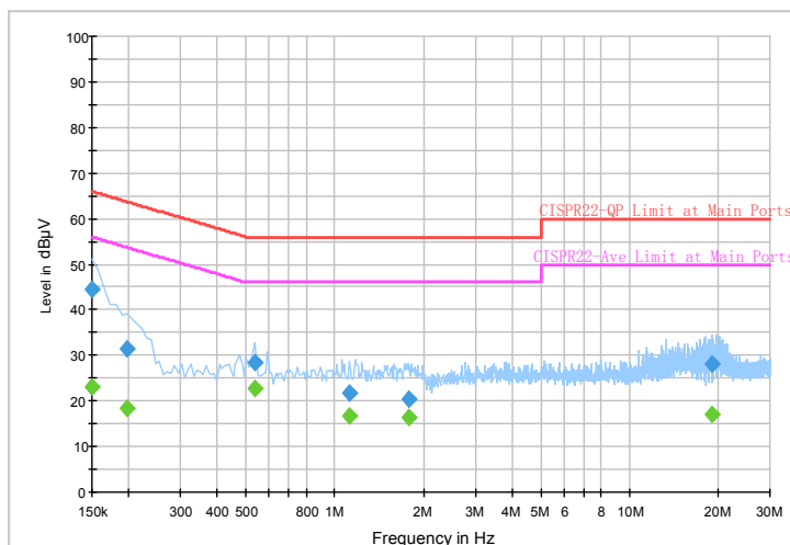
ENV216 Auto Test FCC Power Bar - N
