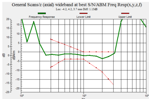
Fig 9.14 WCDMA Band II Ch9400
