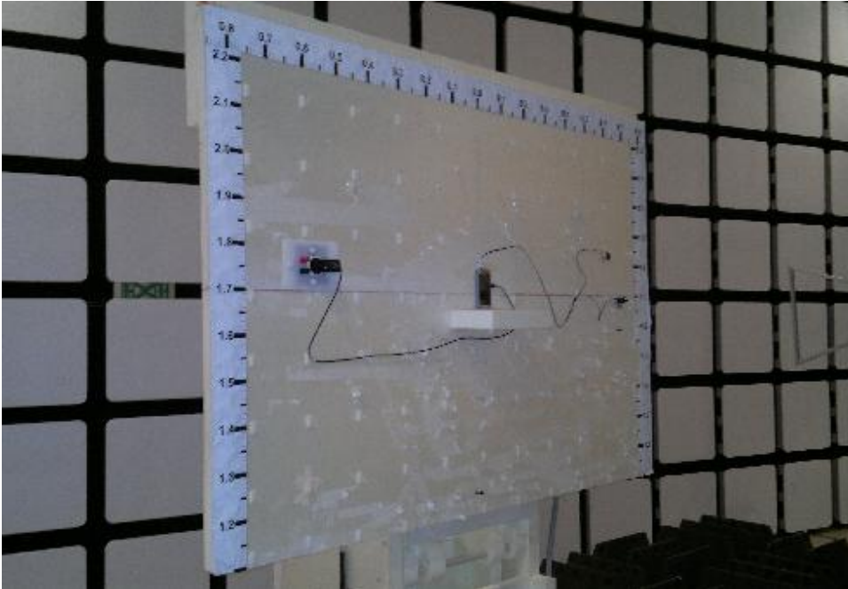
Picture 1. FCC Part 15C Radiated emissions
