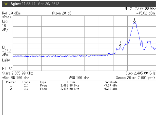
Figure 6. Plot of the Band Edge (Conducted)
