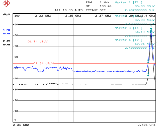
Figure 7. Plot of the Band Edge (Radiated)
