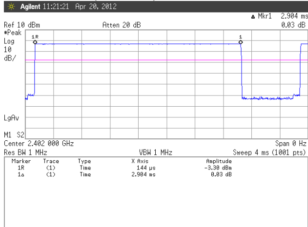
Figure 5. Plot of the Time of Occupancy Basic (GFSK) Lowest Channel (2402 MHz)
