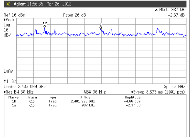
Figure 2. Plot of the Carrier Frequency Separation Basic (GFSK) EDR ( \pi/4 QPSK)
