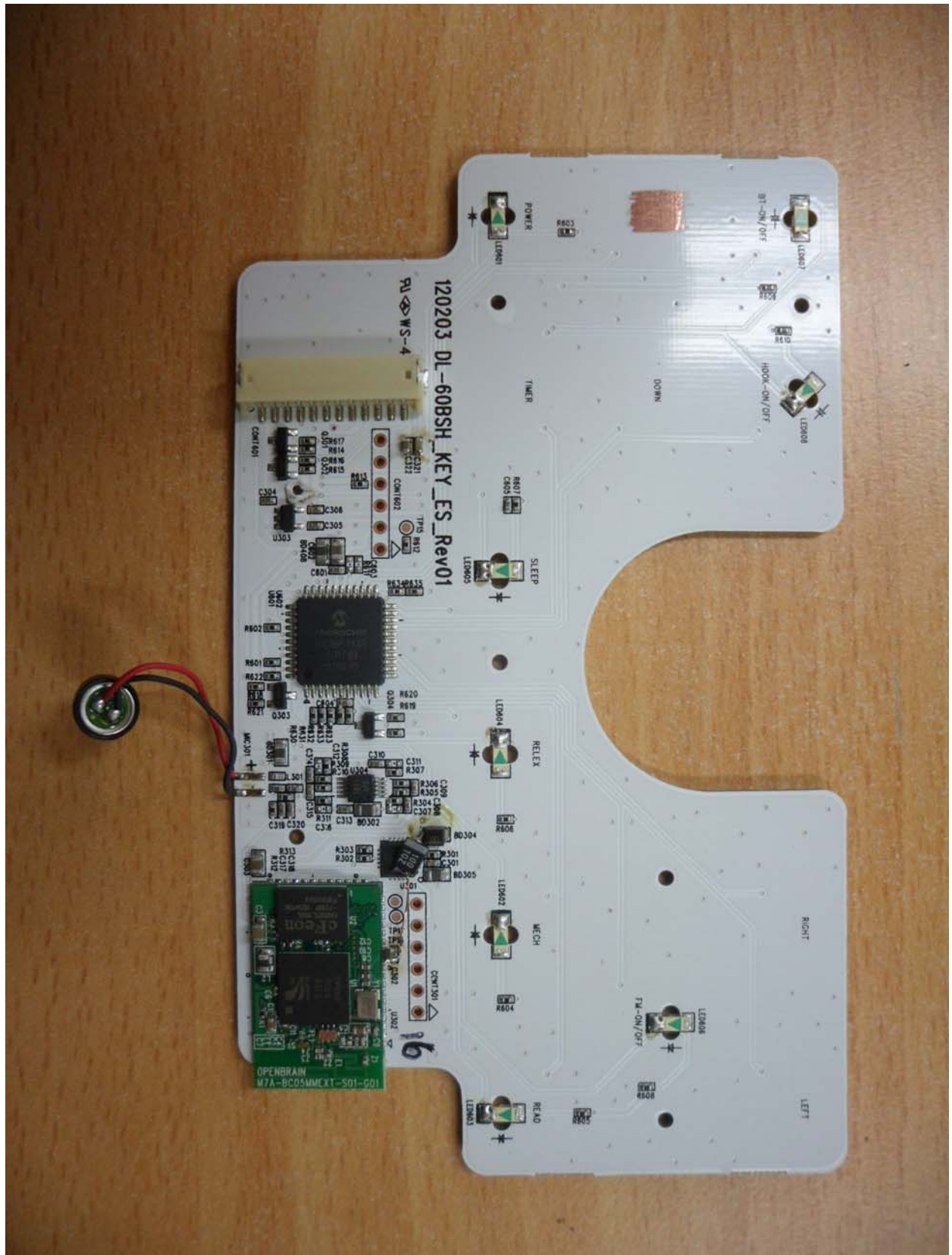
<Photograph 4: Touch board- Front view>
