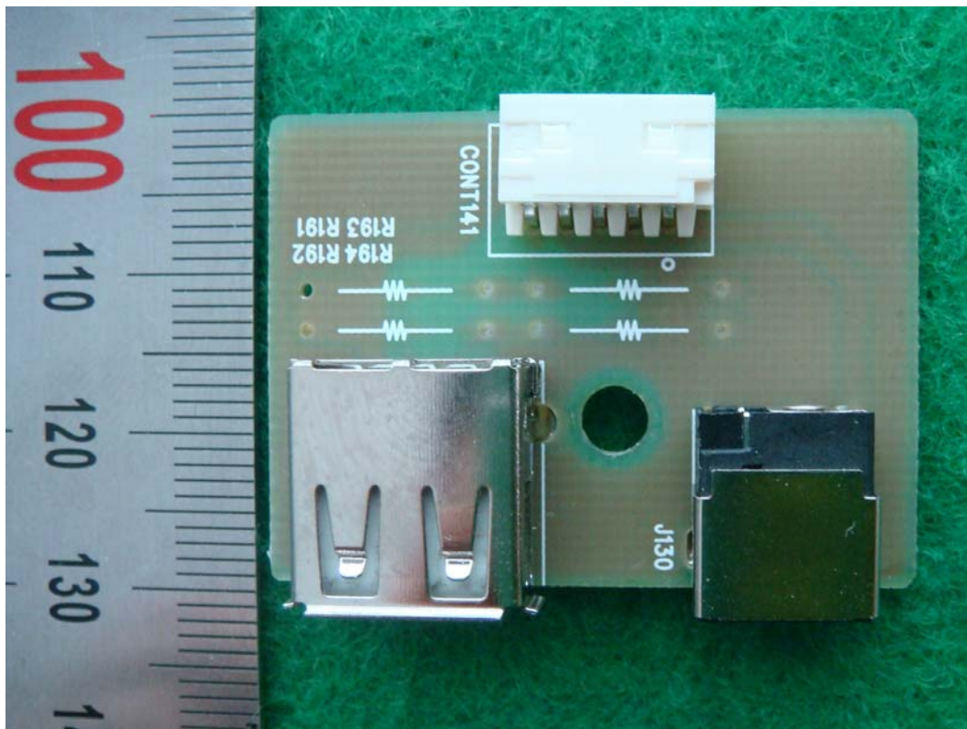
&lt;Photograph 7: Interface board – Front view&gt;
