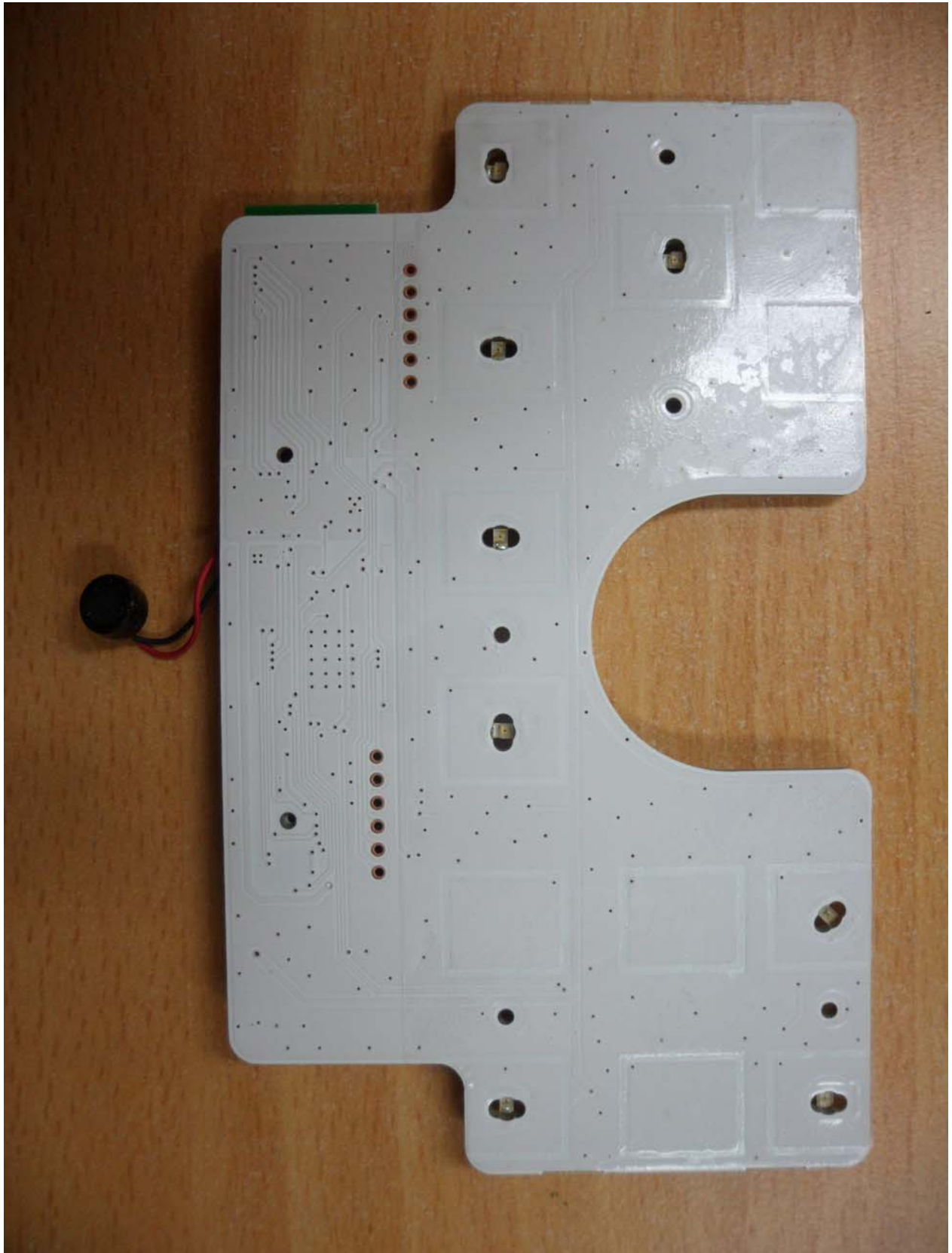
<Photograph 5: Touch board- Rear view>
