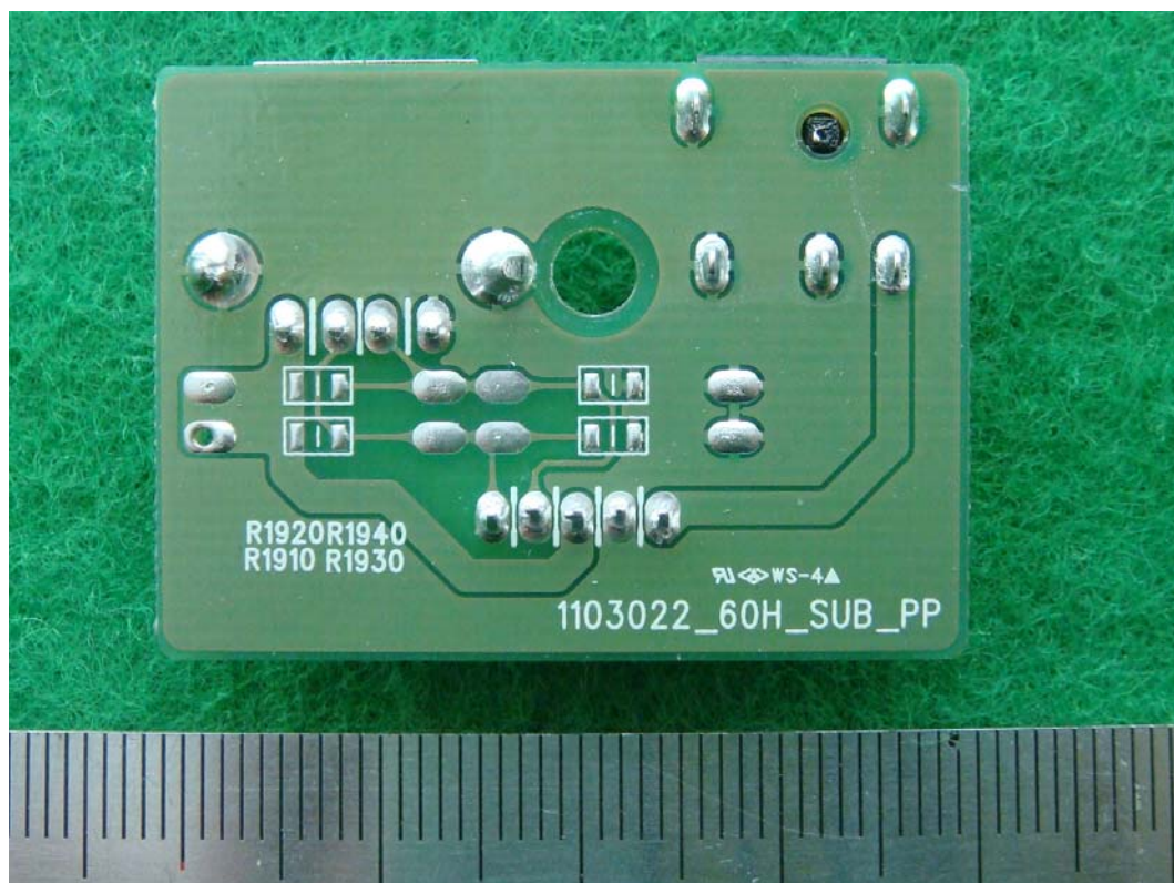
&lt;Photograph 8: Interface board – Front view&gt;
