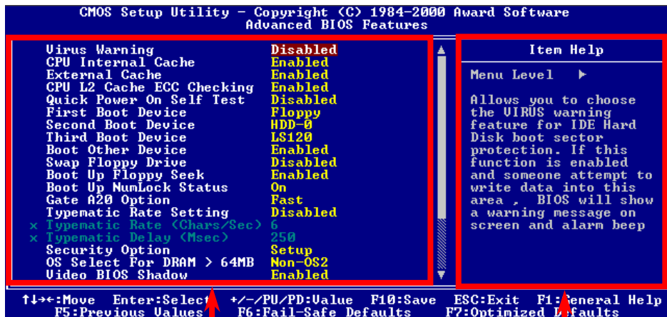
Menu Items Select Window
