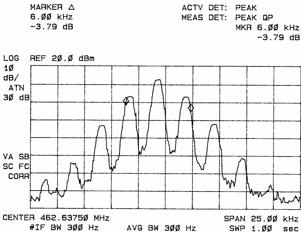
Figure 5: Occupied Band Width.
