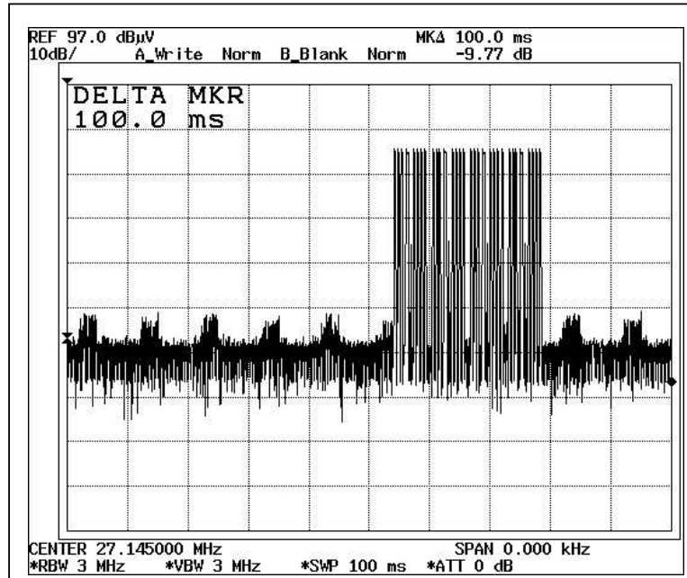
Duty Cycle 1 (Band B)
