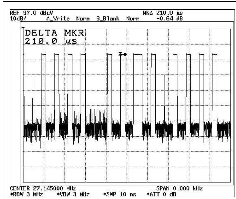
Duty Cycle 3 (Band A)
