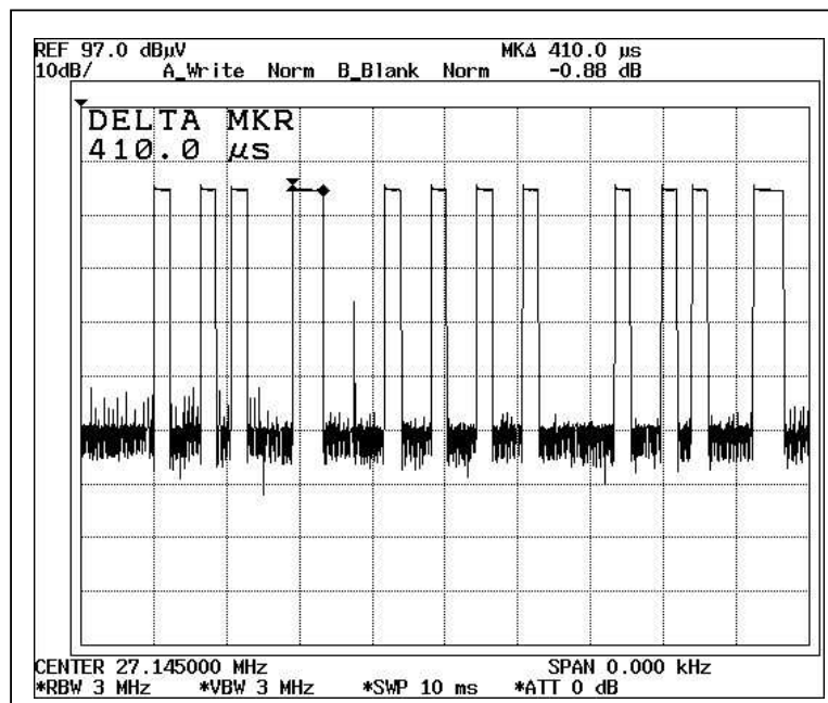
Duty Cycle 2 (Band B)
