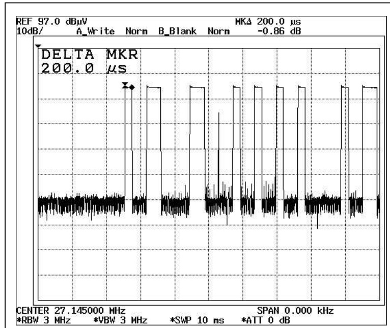
Duty Cycle 3 (Band C)
