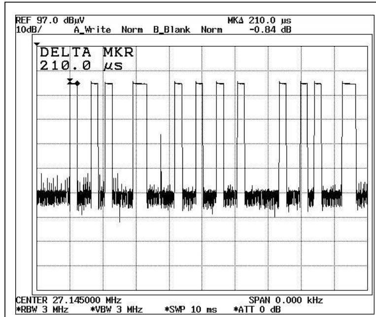
Duty Cycle 3 (Band B)
