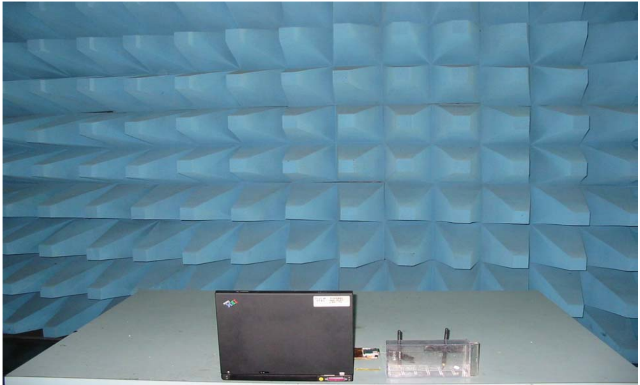
Rear View of the Test Configuration
