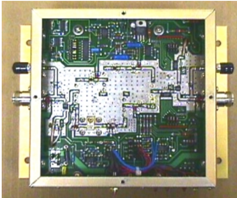
PCS PC BOARD ASSEMBLY
