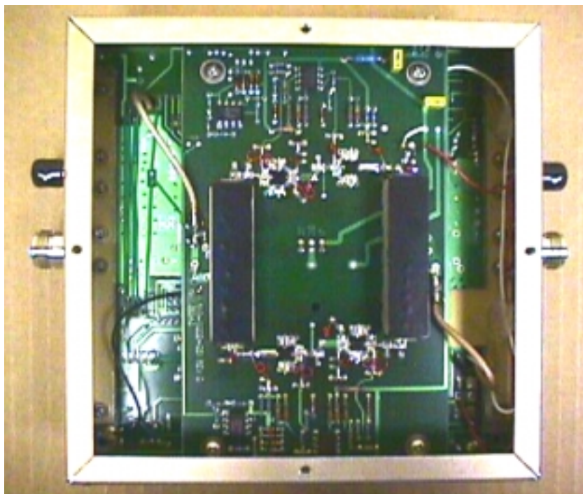
CELLULAR PC BOARD ASSEMBLY
