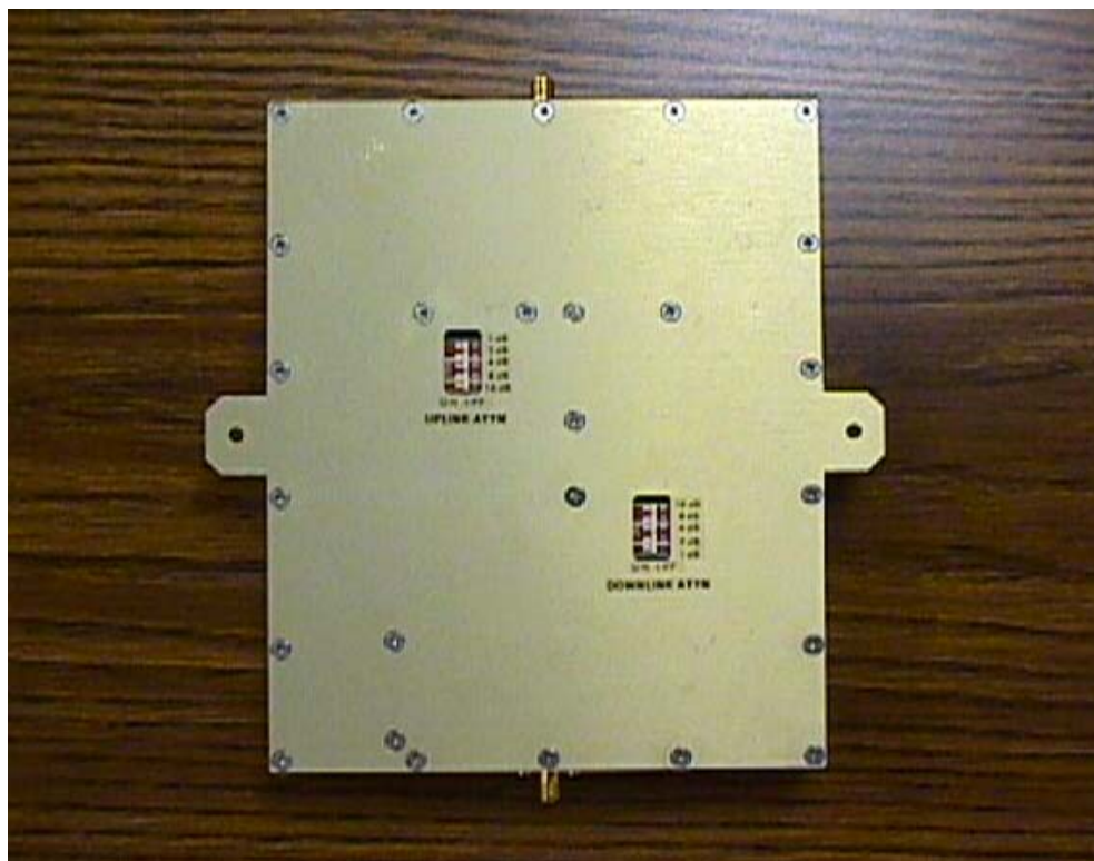
R307B REAR VIEW (MOUNTING SURFACE)
