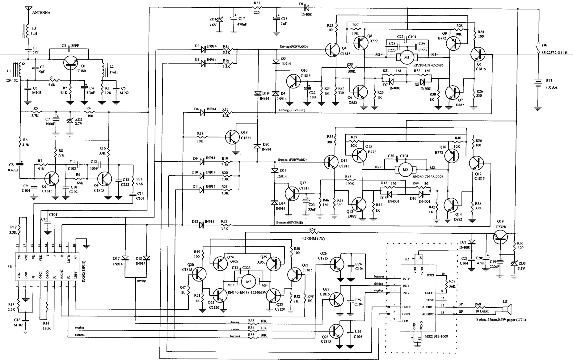
HERALD METAL & PLASTIC WORKS LTD. K'NEX #15128 (49MHZ) RECEIVER CIRCUIT DIAGRAM
