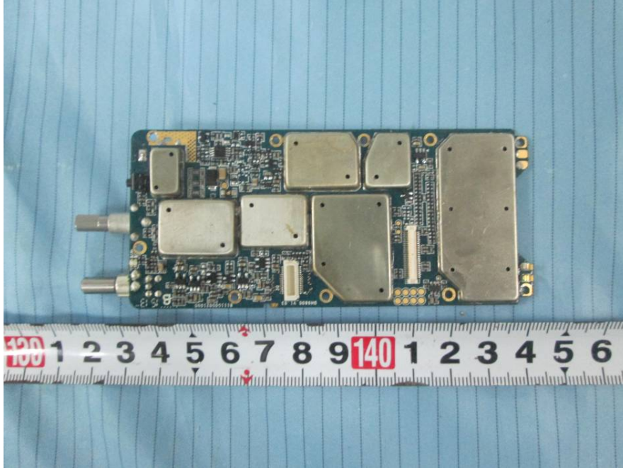
EUT – Main Board 1 Bottom View 3
